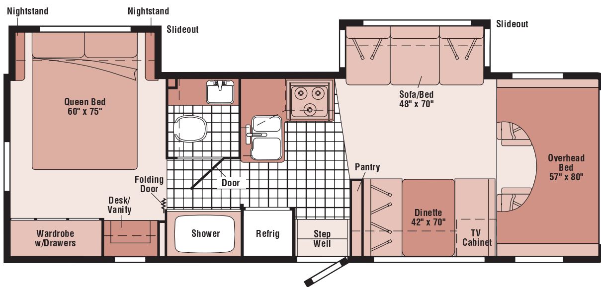
FLOORPLAN
