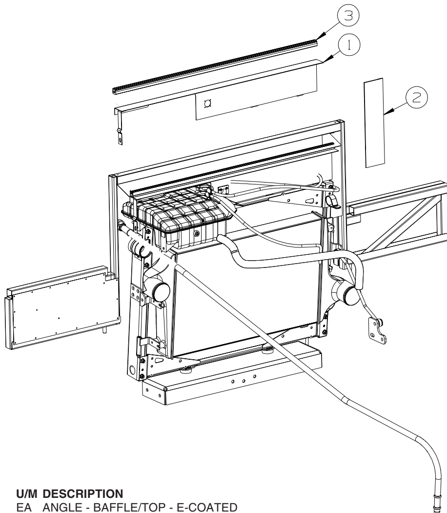
REAR RADIATOR
