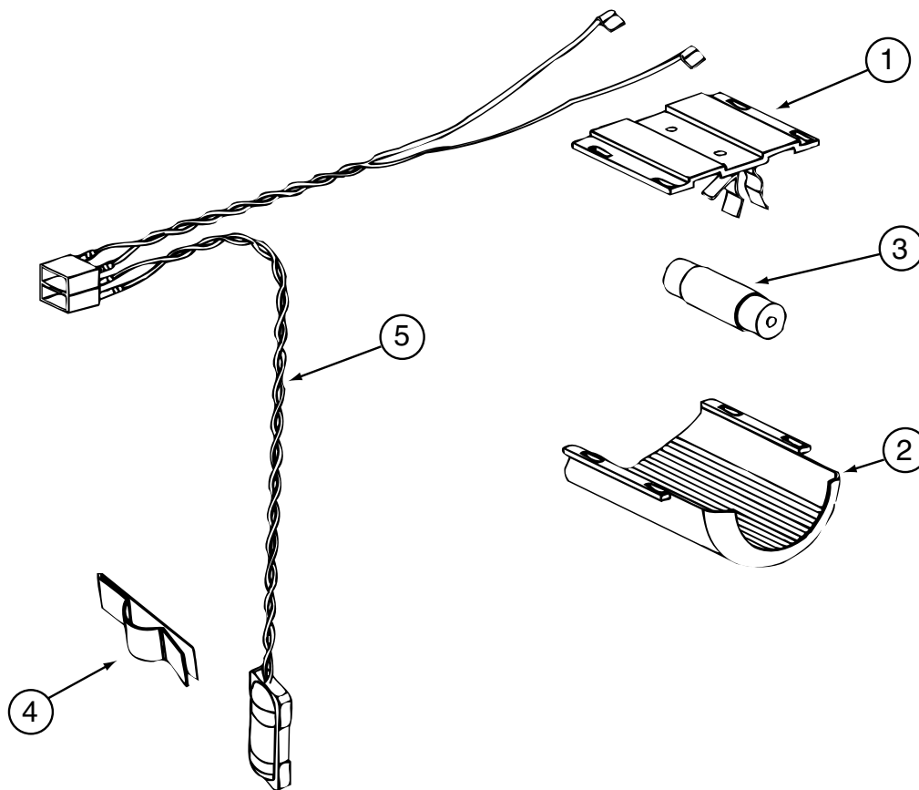
125242-03-01A (CONTINUED)
