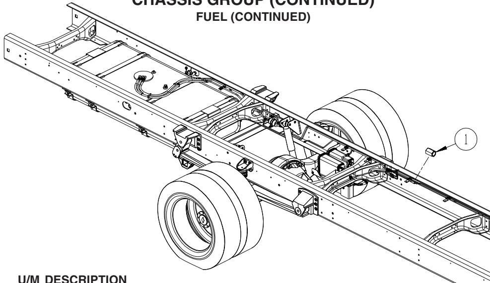
2004 WORKHORSE CHASSIS
