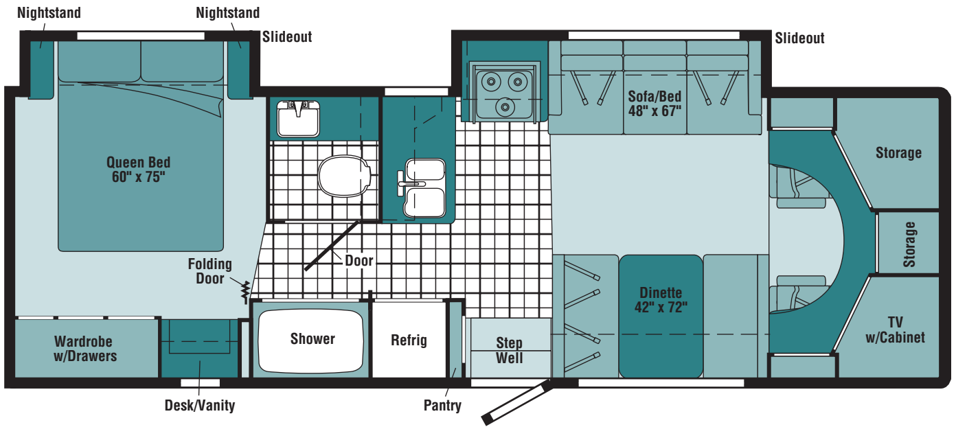
FLOOR PLAN
