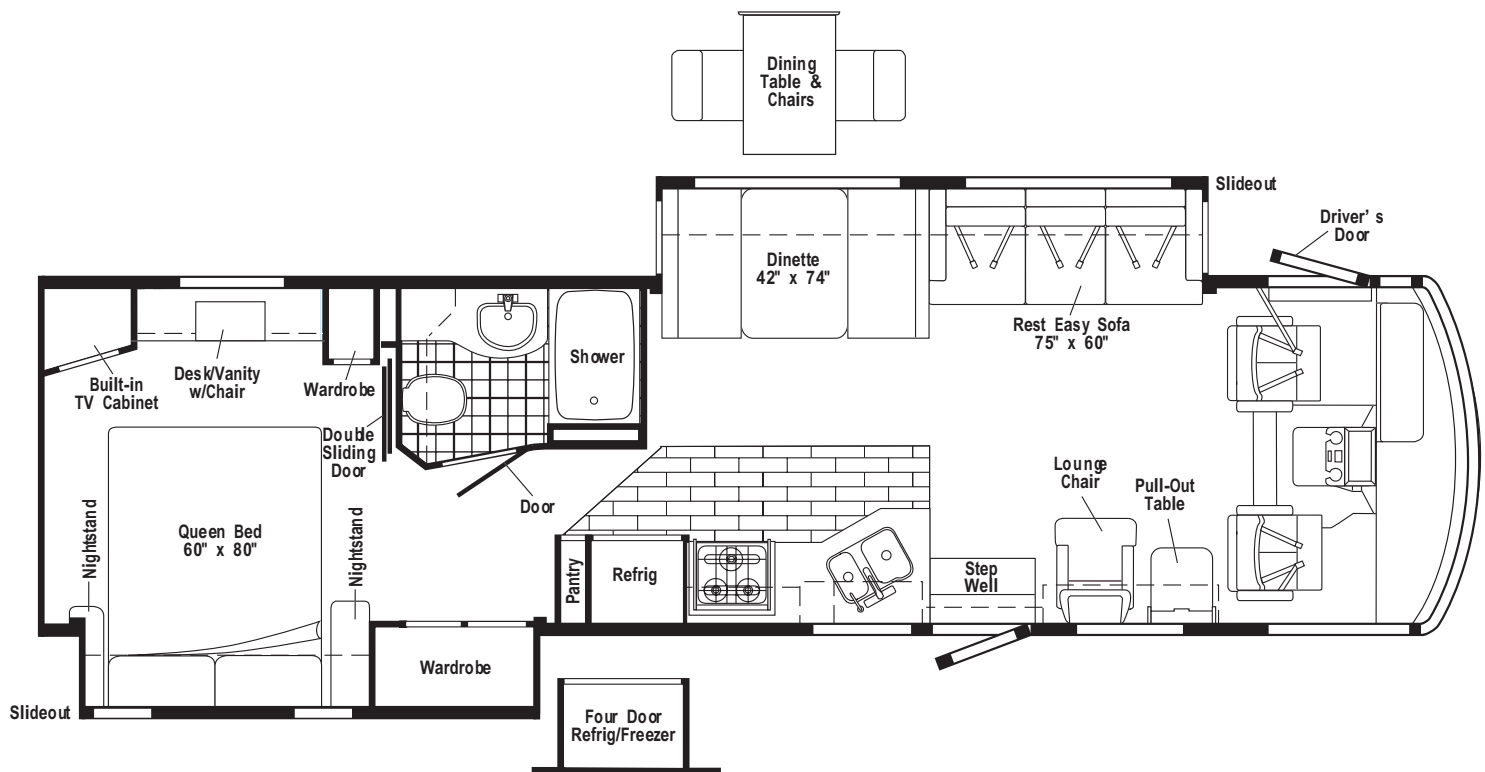
FLOORPLAN
