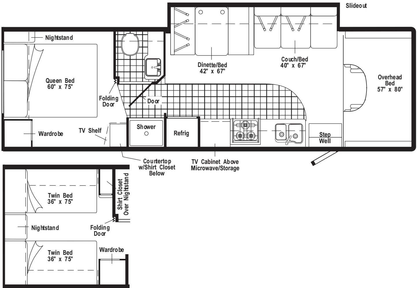
FLOORPLAN
