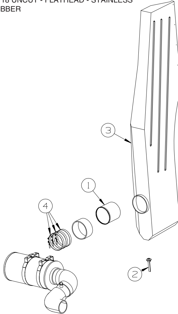
AIR INTAKE
