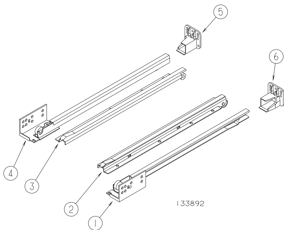
133892 CONCEALED RUNNER DRAWERS
