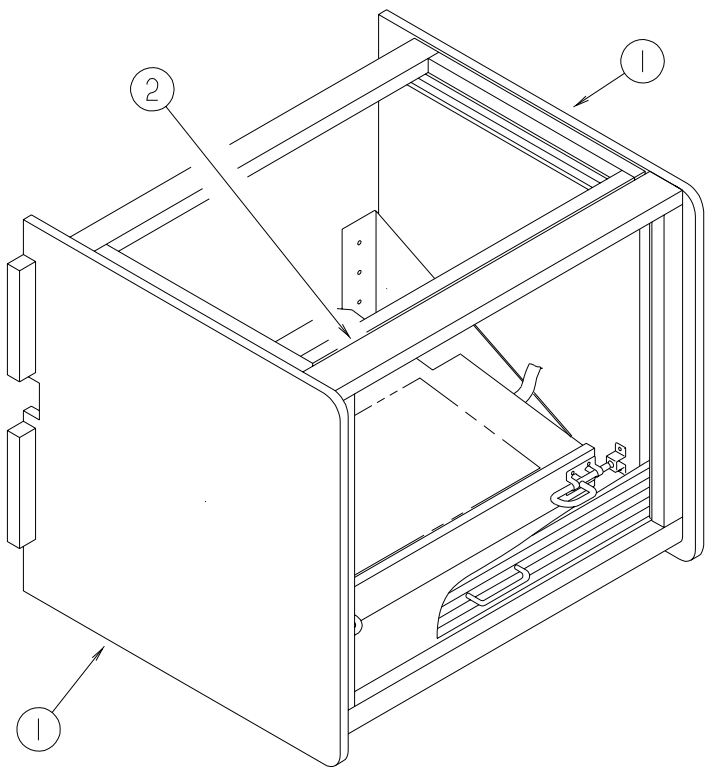
CABINET - W/TV/VCP
