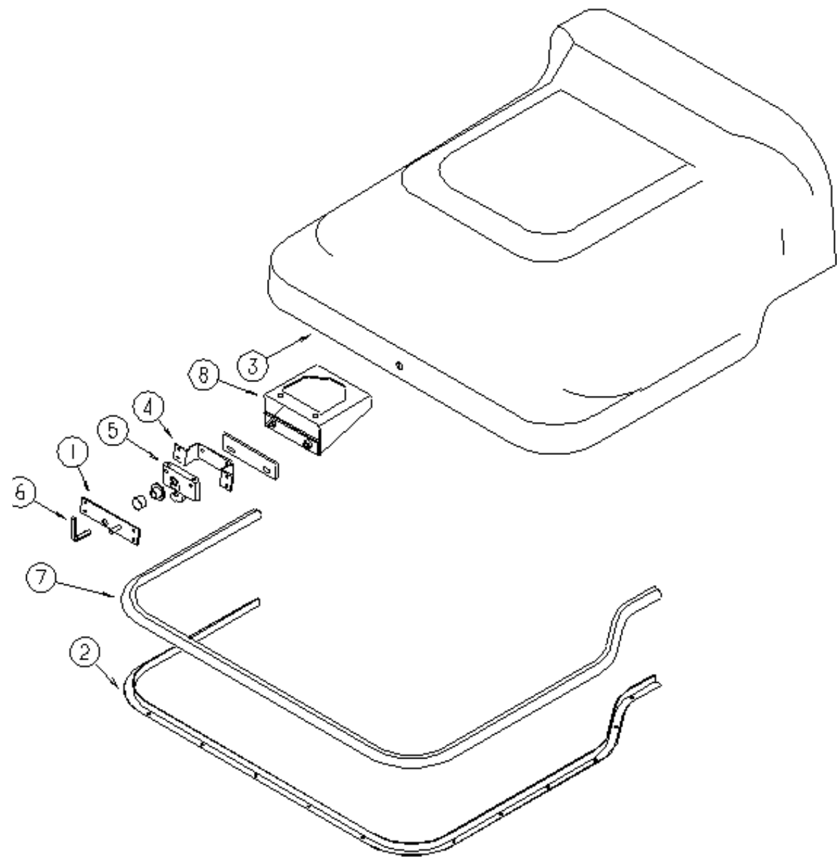
MOTOR COVER
