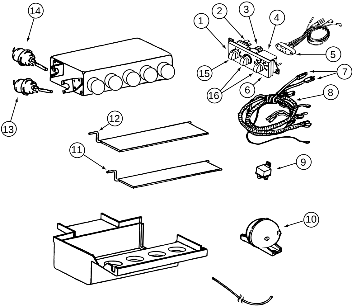
CONTROL & PLENUM
