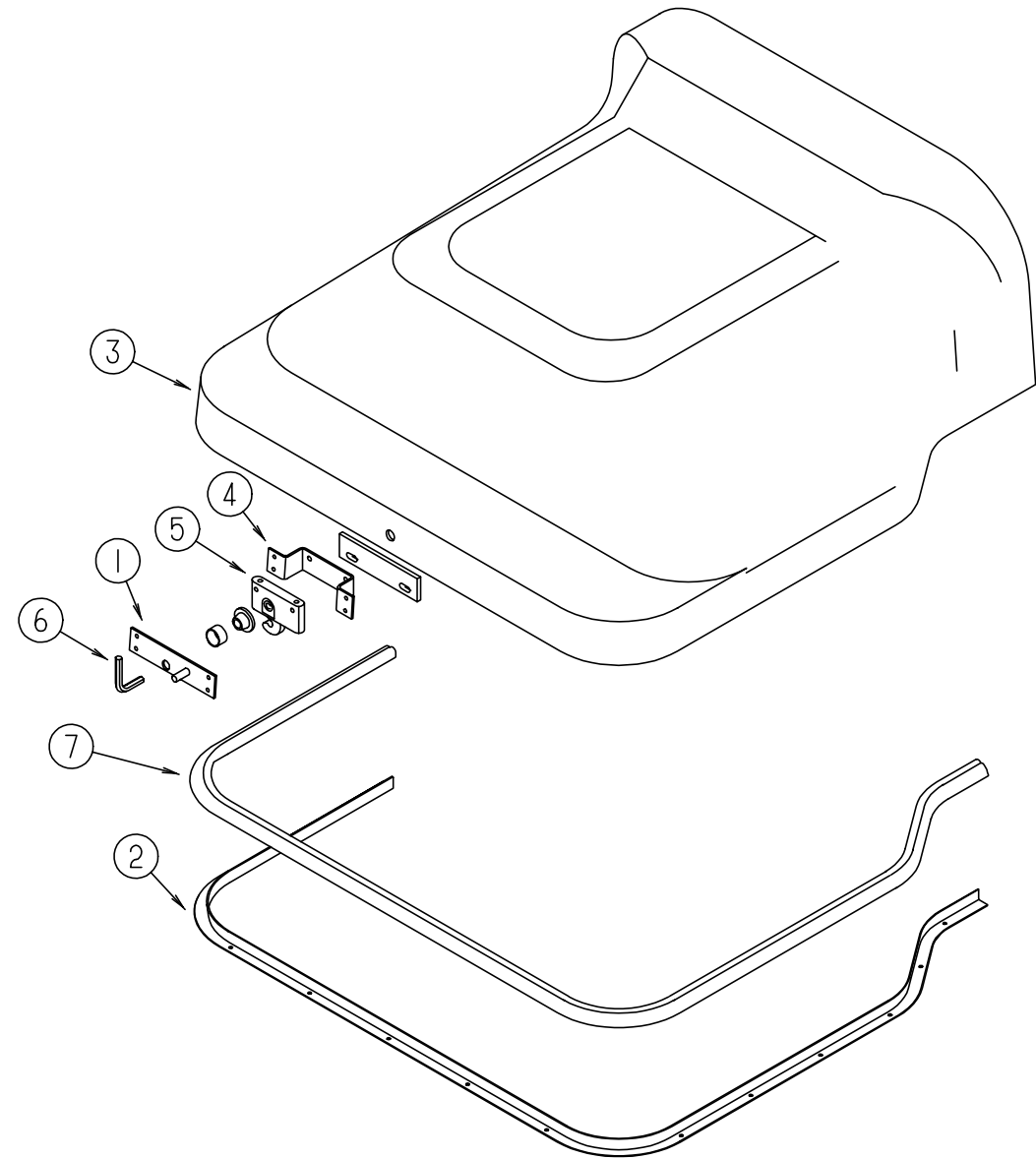
MOTOR COVER
