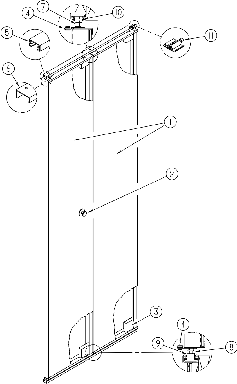
QUEEN BED WARDROBE DOOR FROM: 00-00-00 THRU: 01-11-98
