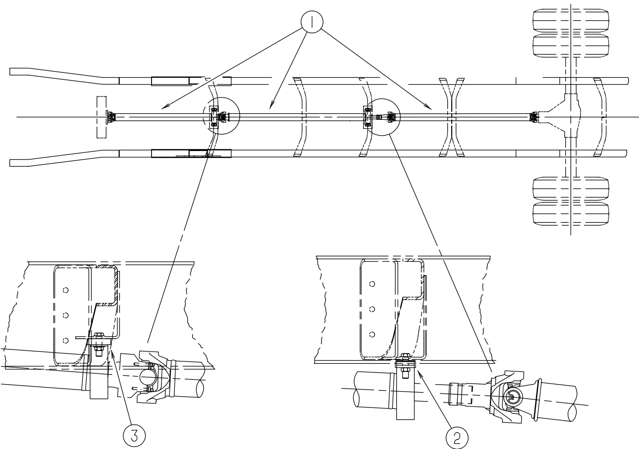
FORD DRIVETRAIN
