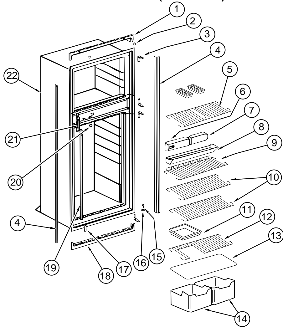
NORCOLD MODEL 982 REFRIGERATOR CABINET ASM WITH TRAY, TIEDOWNS, & LEVEL
