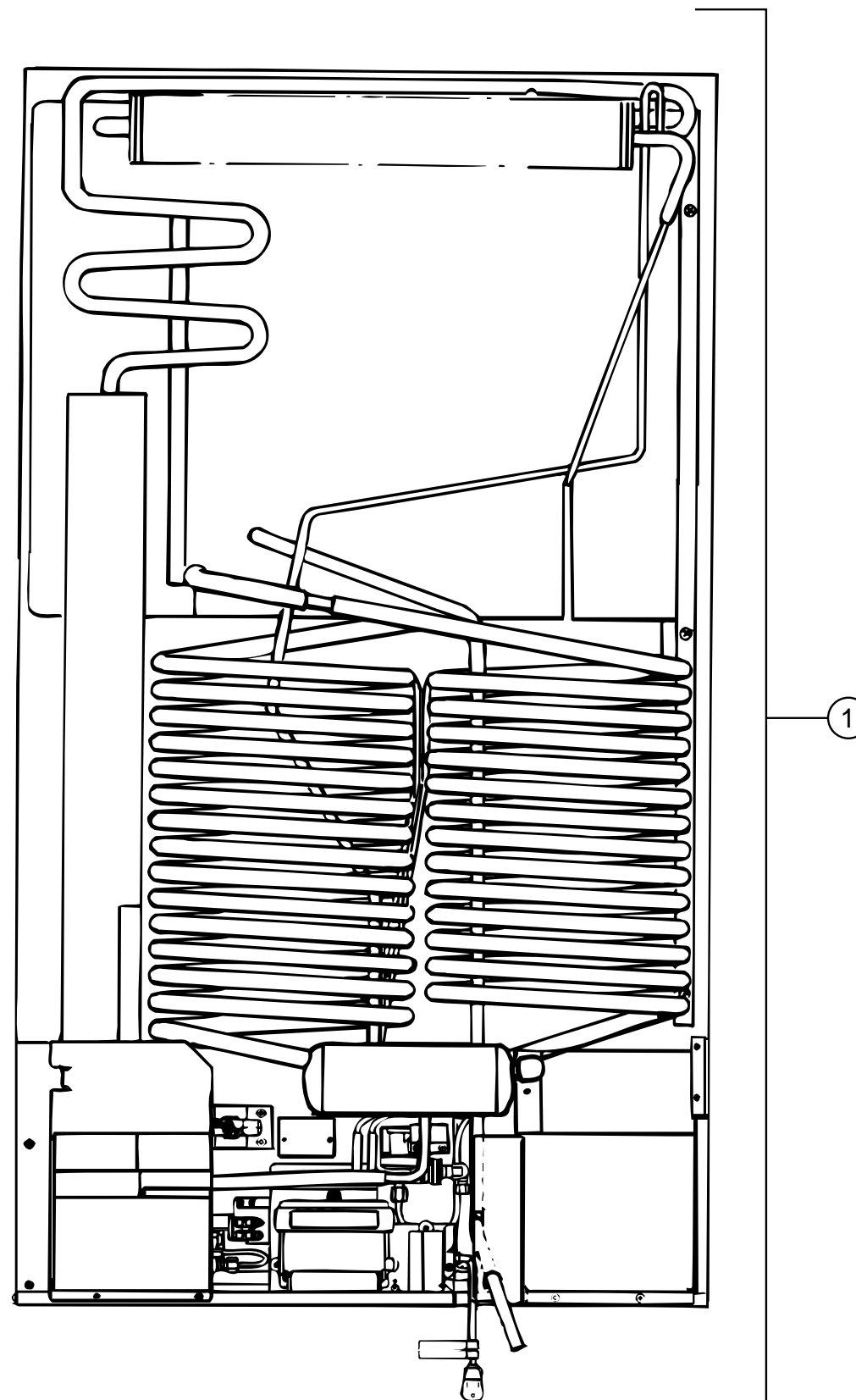
DOMETIC RM 7732IM REFRIGERATOR COOLING COIL
