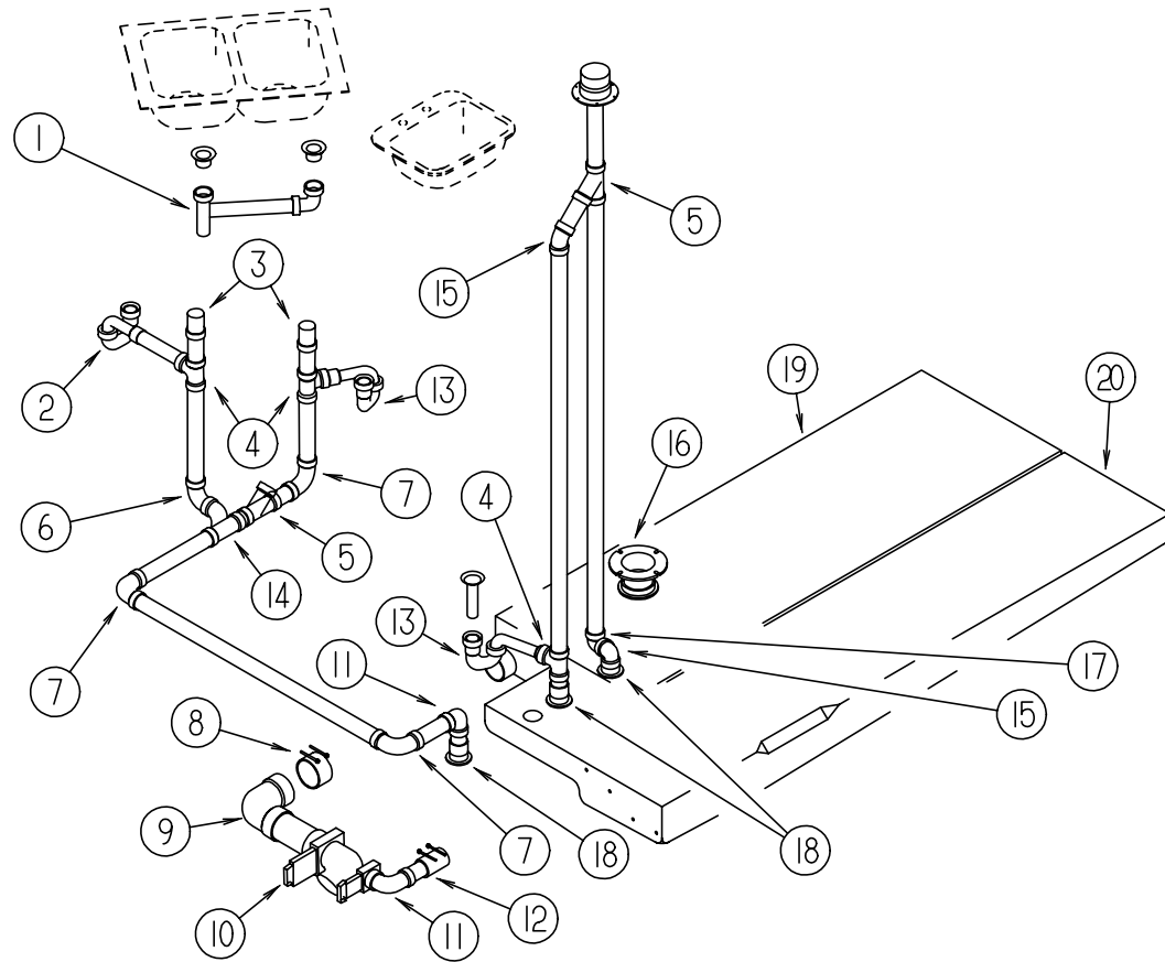
DRAINAGE SYSTEM
