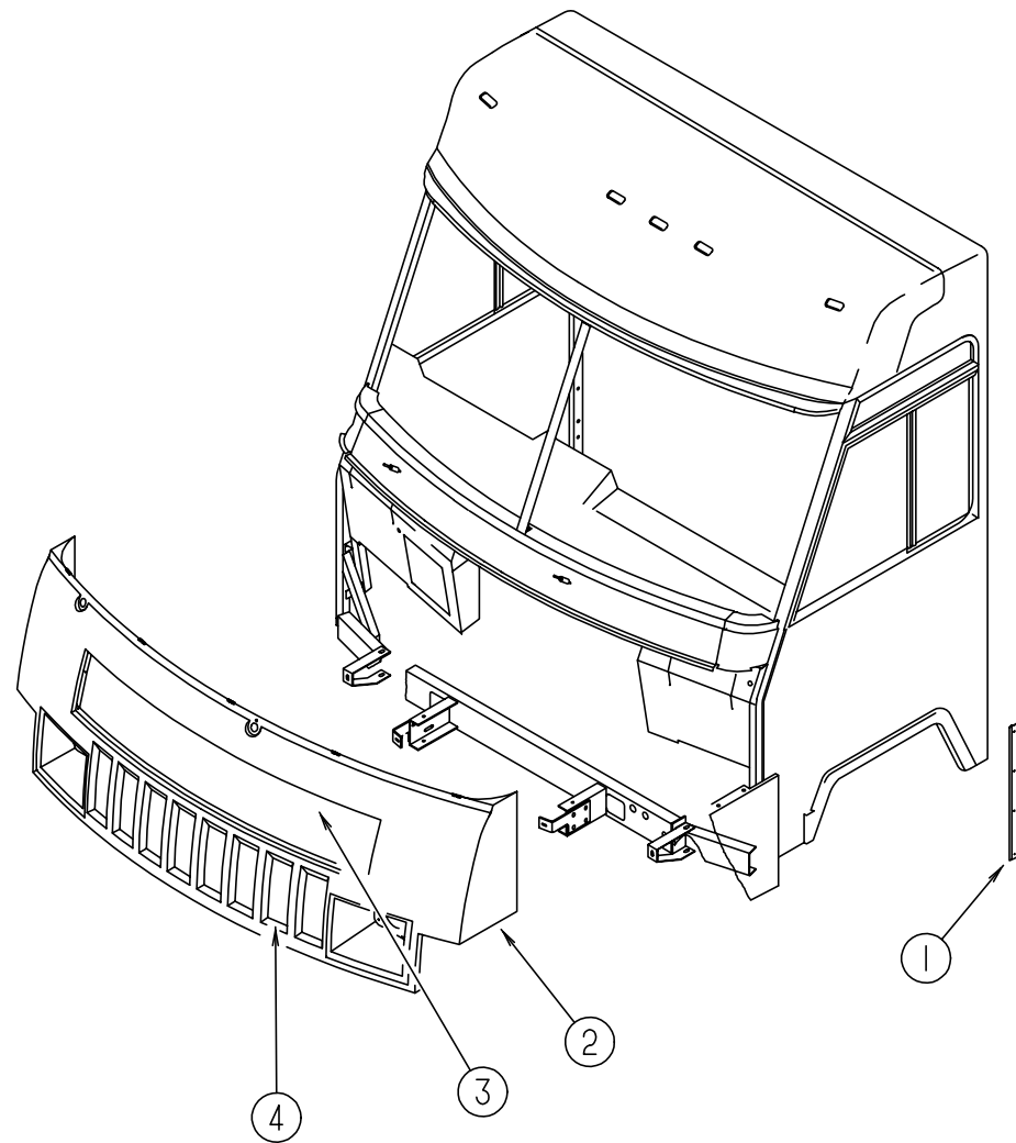
FRONT END ASSEMBLY
