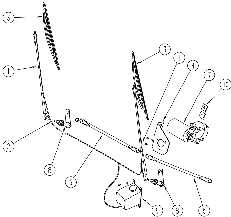
WIPER COMPONENTS
