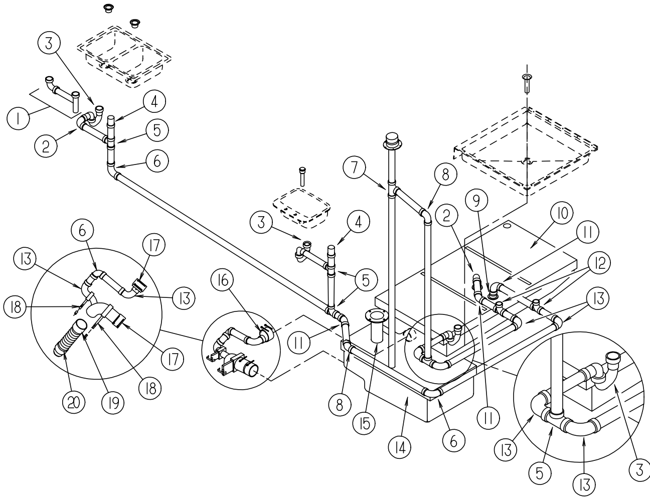
DRAINAGE SYSTEM
