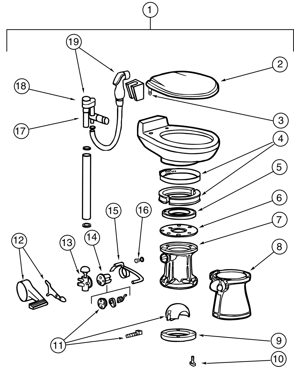
TOILET (SEALAND)
