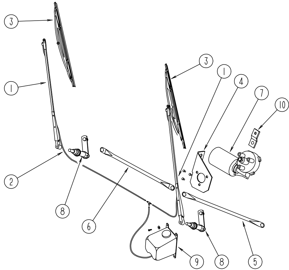
WIPER COMPONENTS
