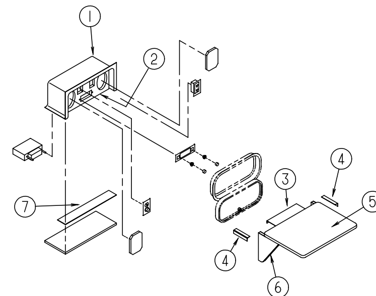
EXTERIOR ENTERTAINMENT CENTER
