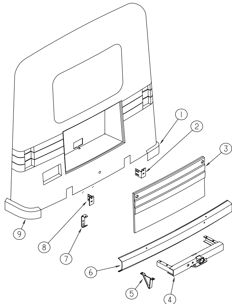
REAR BUMPER, END CAPS & TRAILER HITCH
