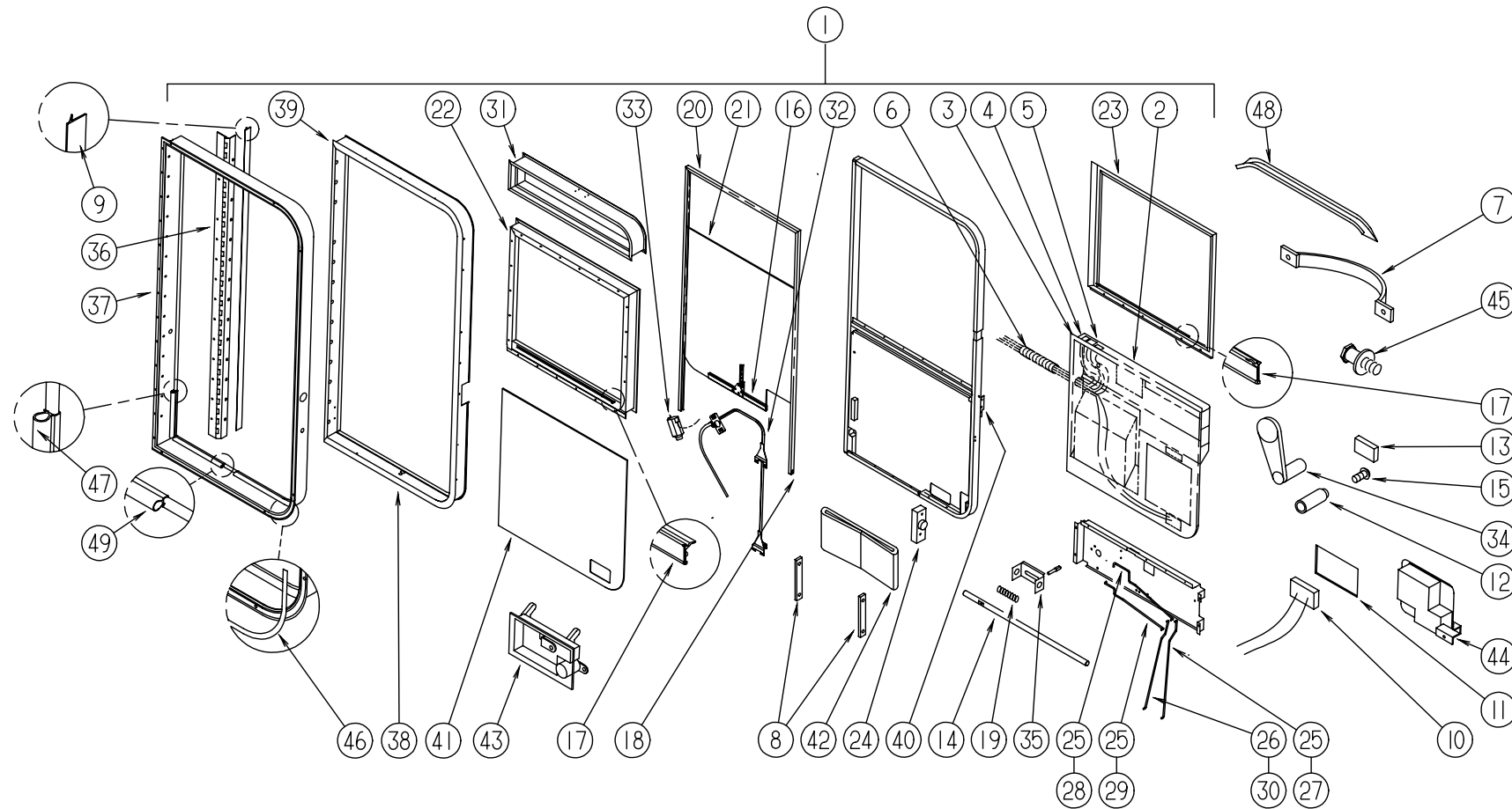
DRIVERS DOOR & COMPONENTS (CONTINUED)
