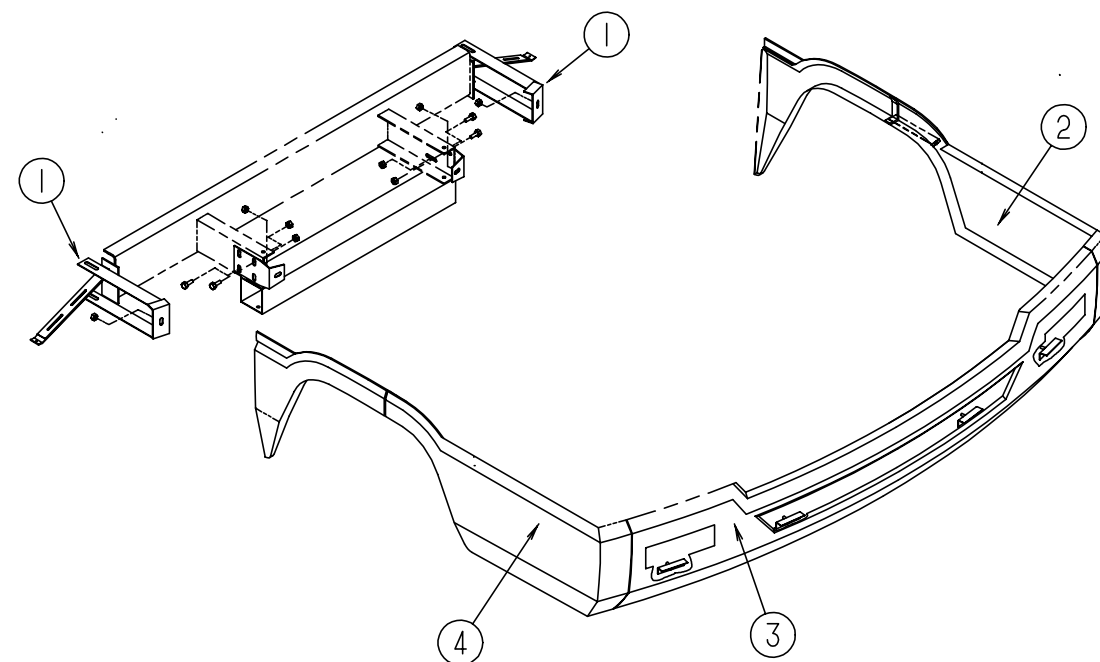
FRONT BUMPER & PANELS
