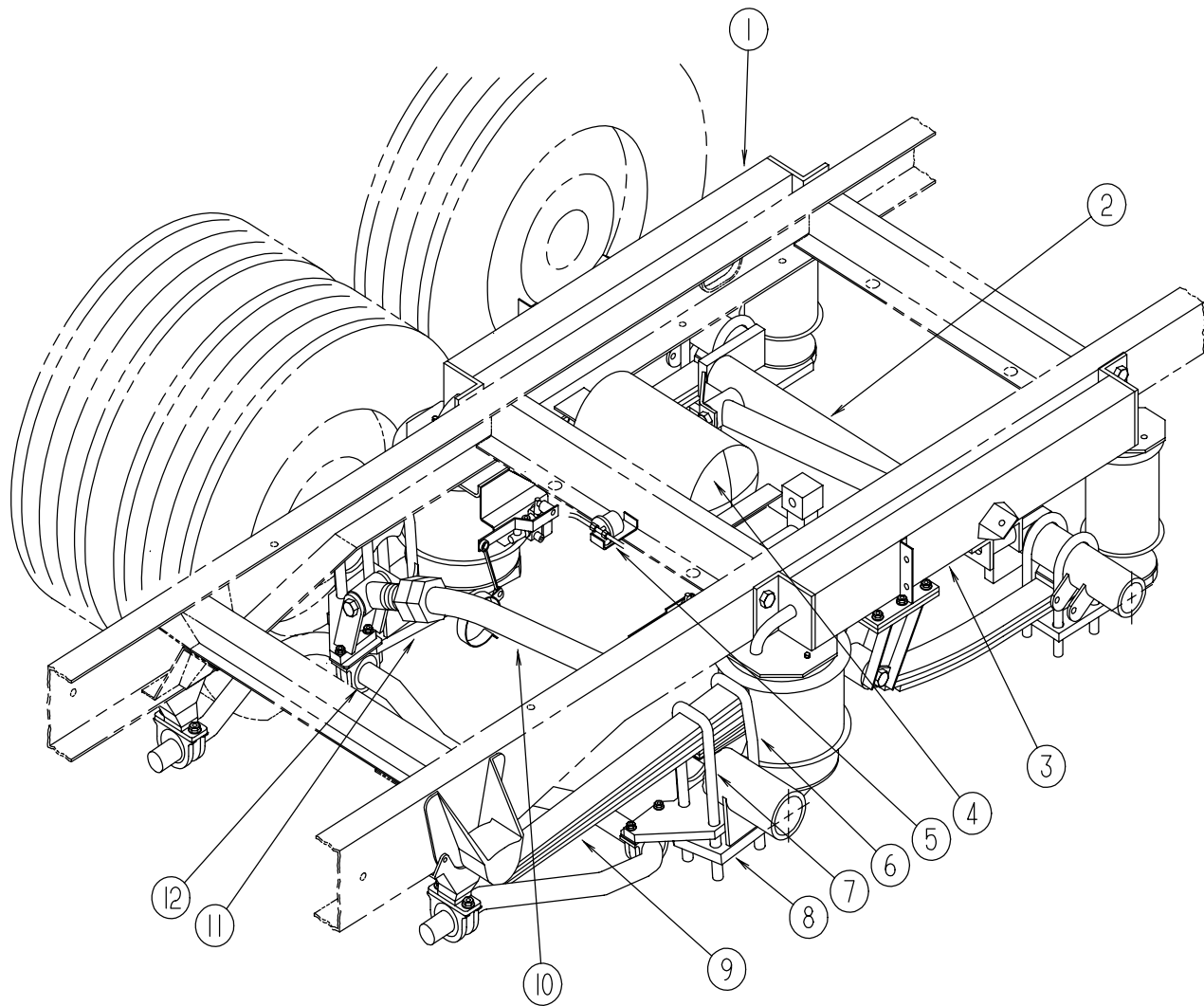
CHEVY JET AIR TAG AXLE
