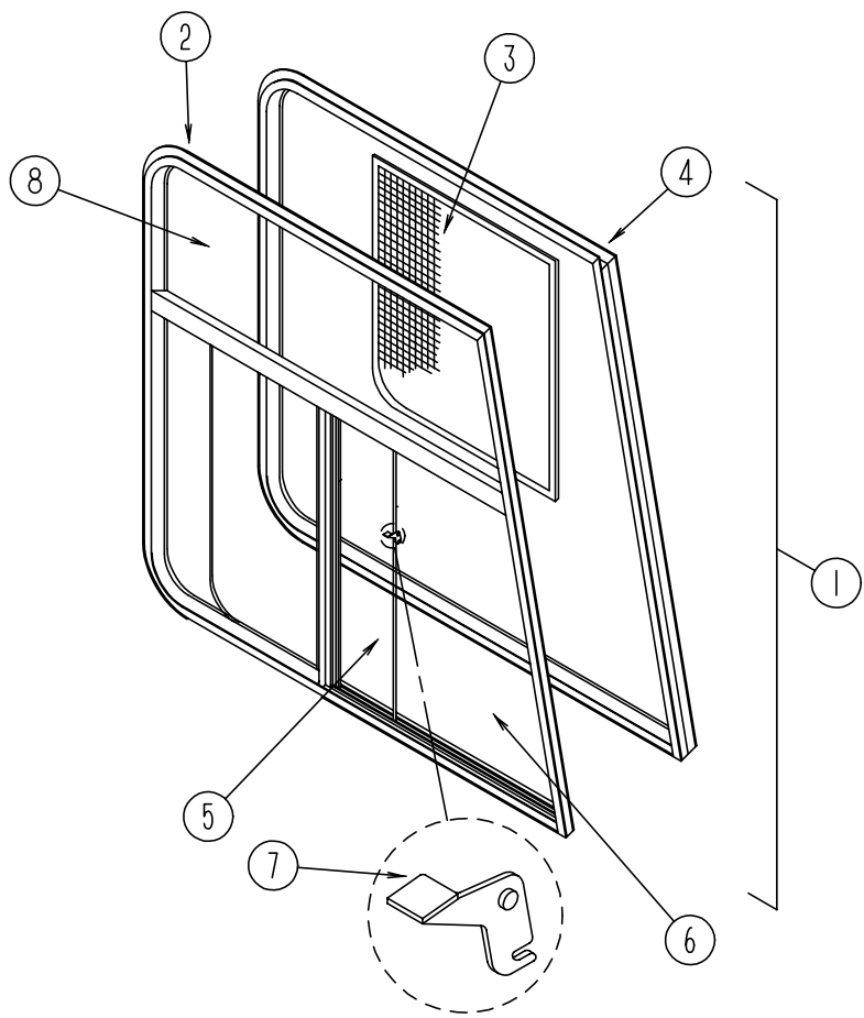
DRIVER & PASSENGER CAB SIDE WINDOWS FROM: 00-00-00 THRU: 09-11-93
