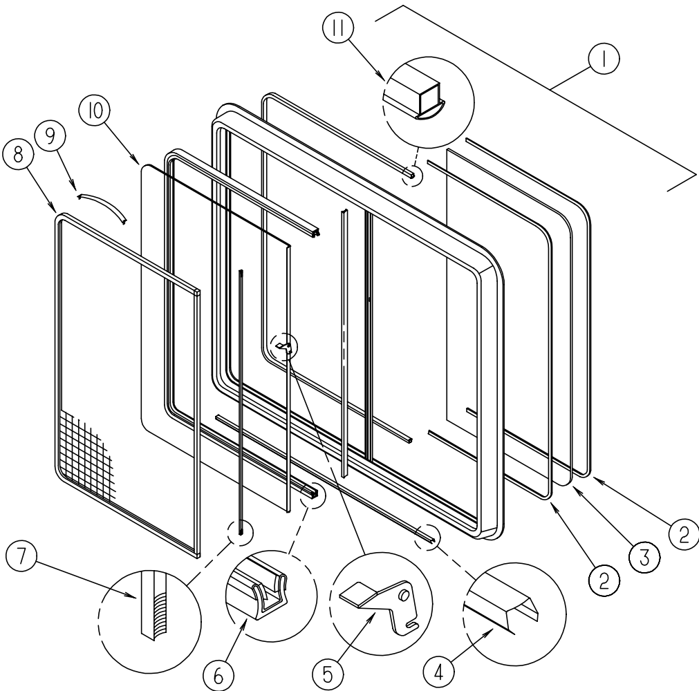
GALLEY SLIDING WINDOW
