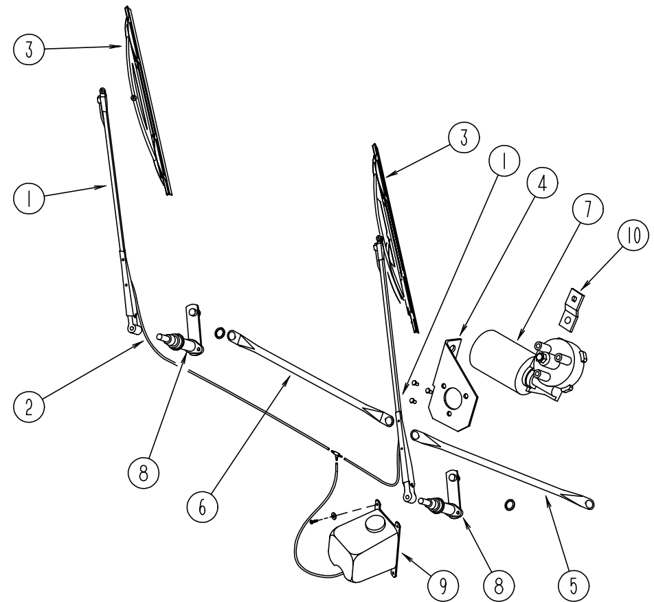
WIPER COMPONENTS
