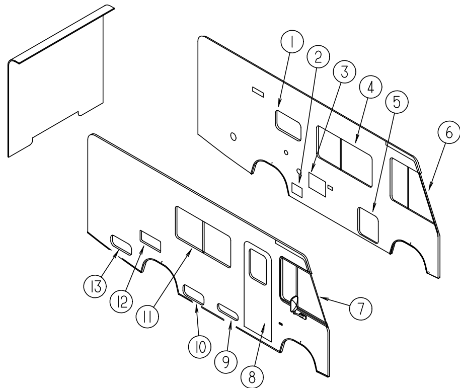
EXTERIOR WINDOWS & DOORS
