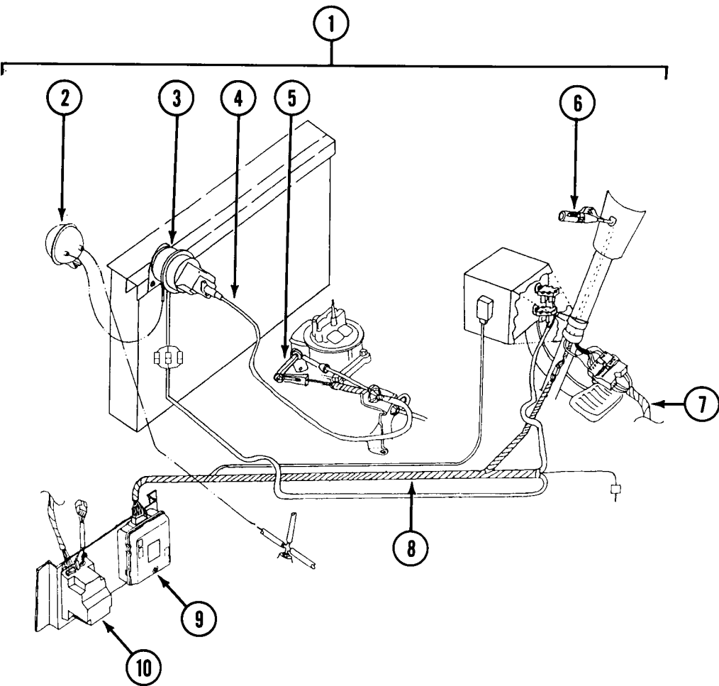
SPEED CONTROL FOR 1993 CHEVY CHASSIS ONLY (GAS)
