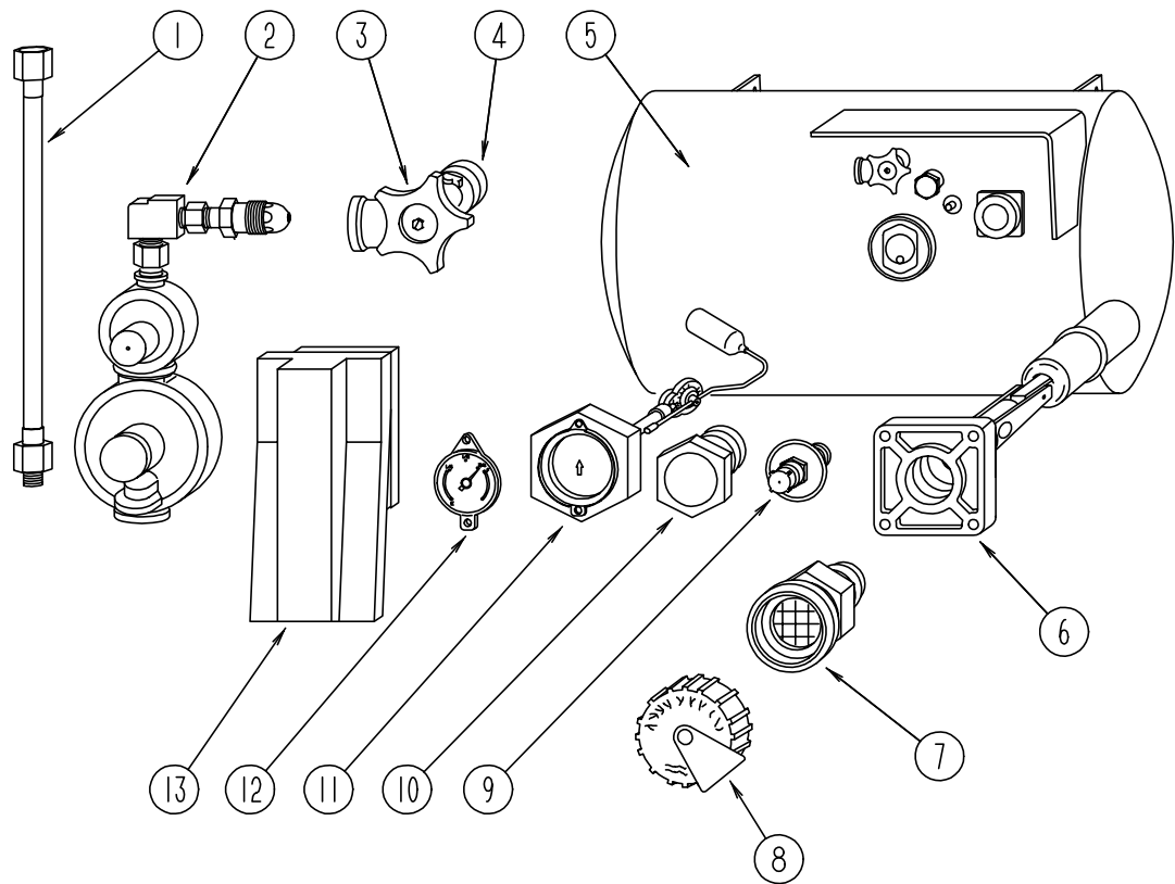
LP TANK & SYSTEM COMPONENTS
