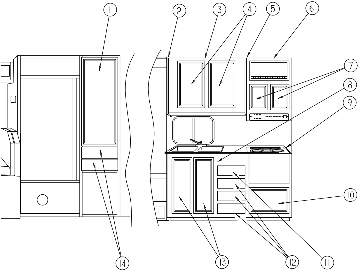
GALLEY CABINETS & FIXTURES
