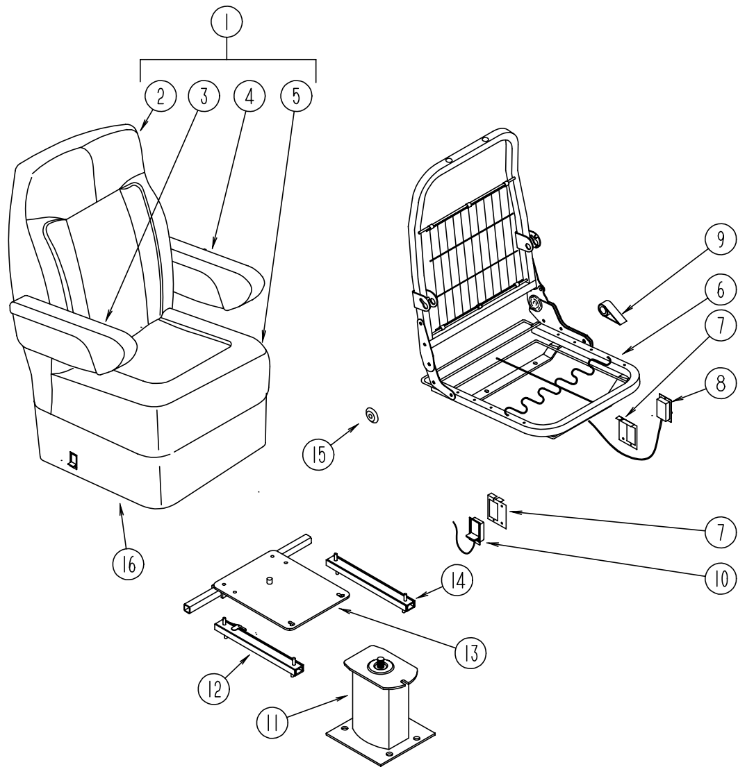
FORD BUCKET SEATS (CONTINUED)
