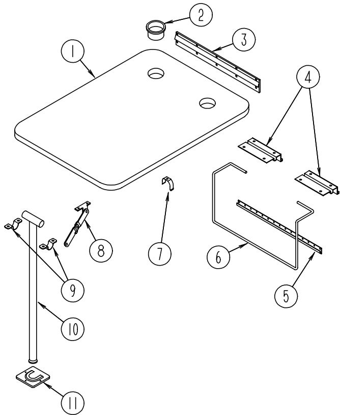
DINETTE TABLES & HARDWARE
