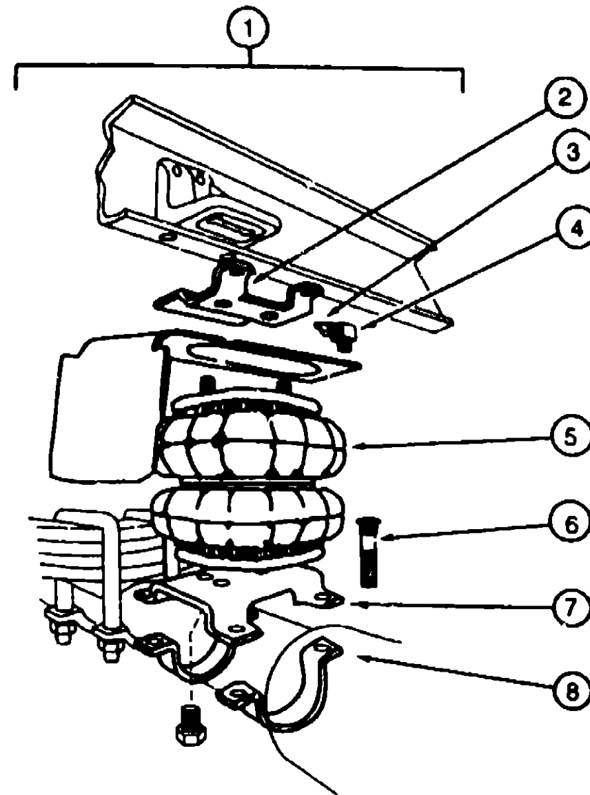
REAR AXLE AIRSPRING, CHEVY (FIRESTONE) (FROM: 00-00-00 THRU: 09-29-92)
