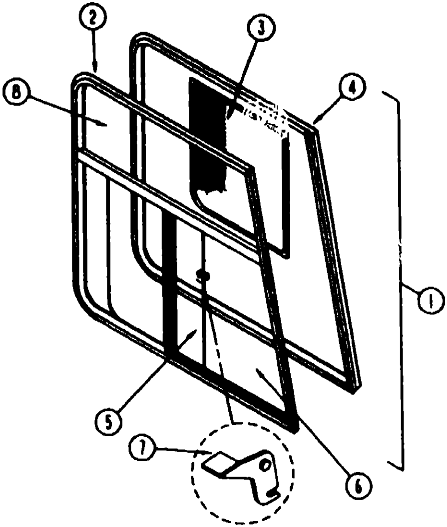
FRONT CAB WINDOWS (EXCEL) (FROM: 00-00-00 THRU: 07-19-82)
