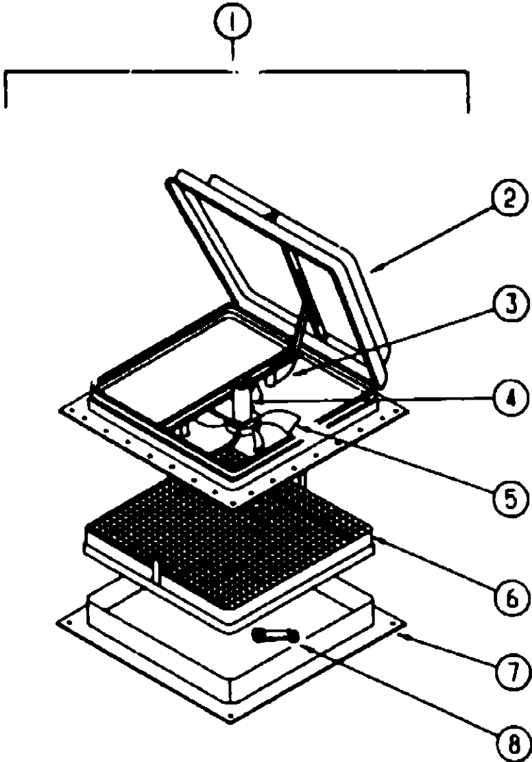
POWERED ROOF VENT (CANADIAN) (1" ROOF)
