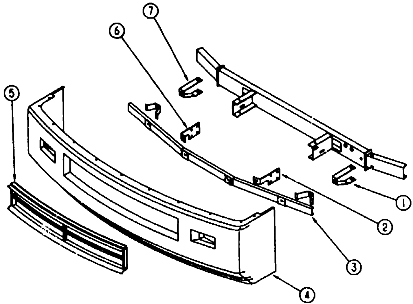
FRONT BUMPER
