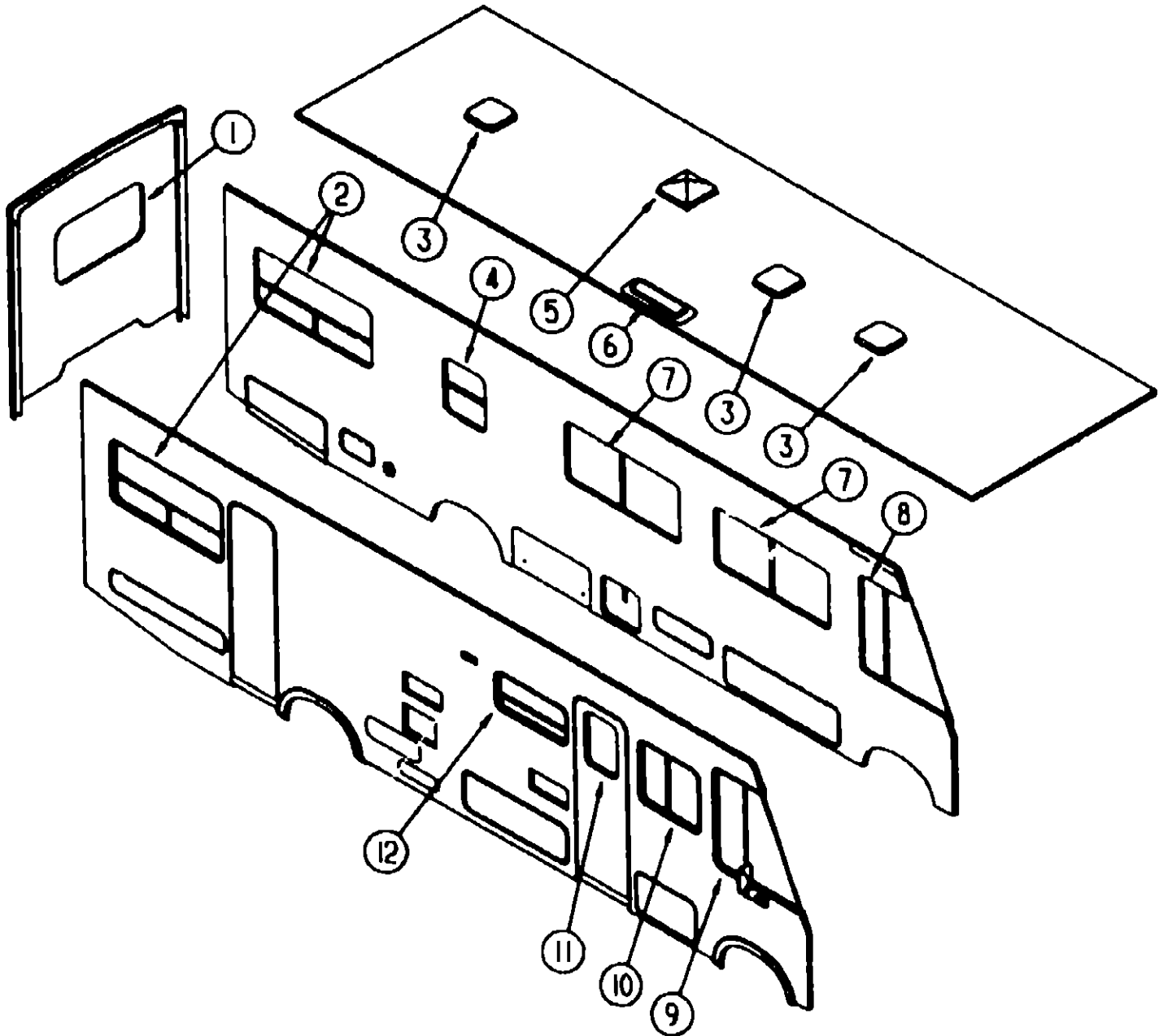
WINDOWS & VENTS
