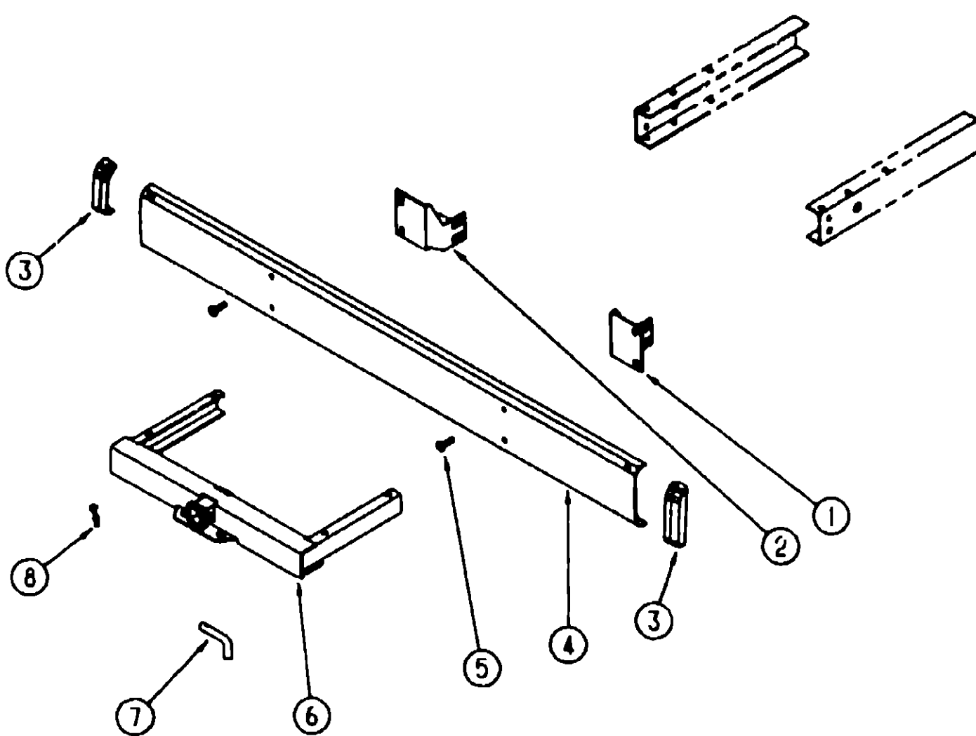
REAR BUMPER
