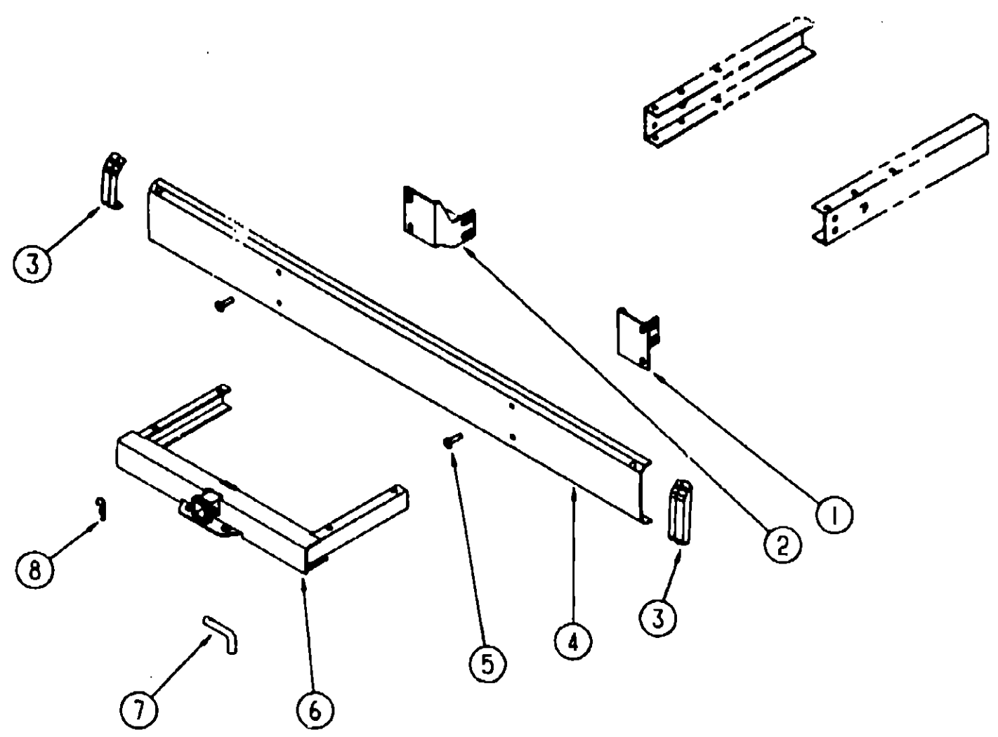
REAR BUMPER
