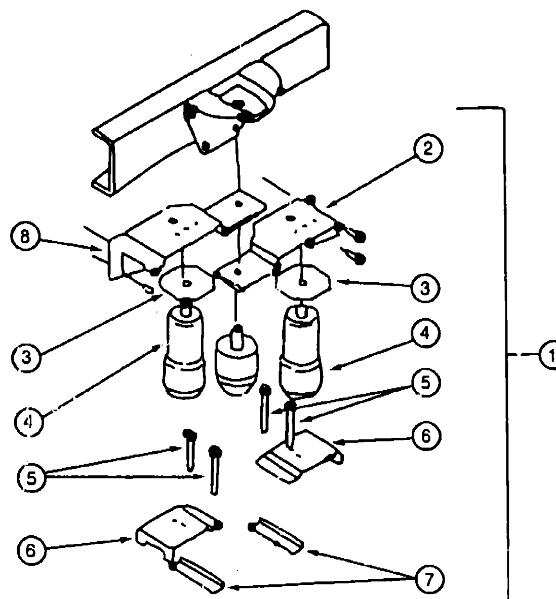
REAR AXLE AIRSPRING,CHEVY (RIDE RITE) (FROM: 10-02-92 THRU: 99-99-99)
