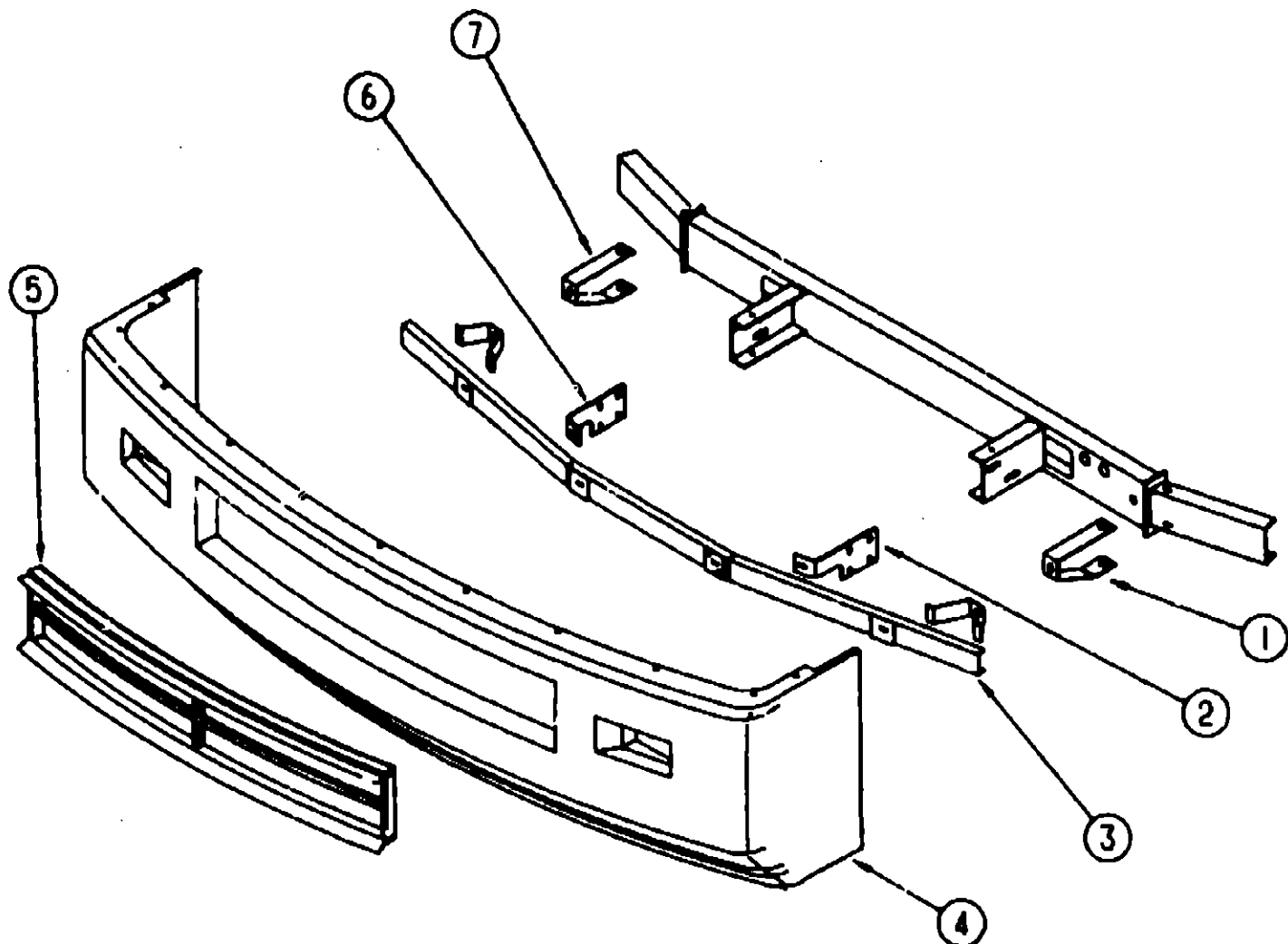
FRONT BUMPER
