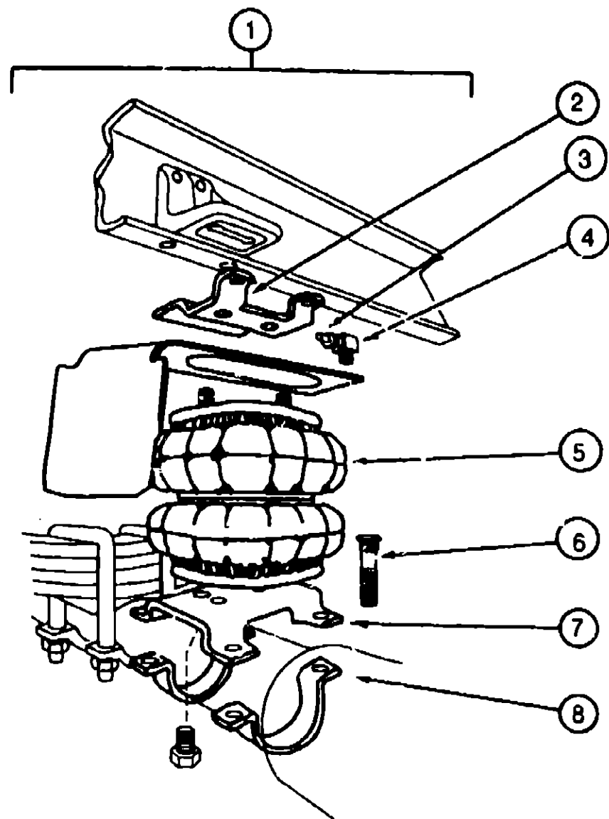
REAR AXLE AIRSPRING,CHEVY (FIRESTONE) (FROM: 00-00-00 THRU: 10-02-92)
