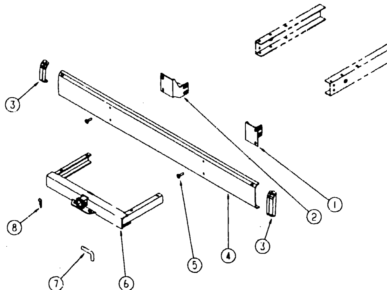
REAR BUMPER
