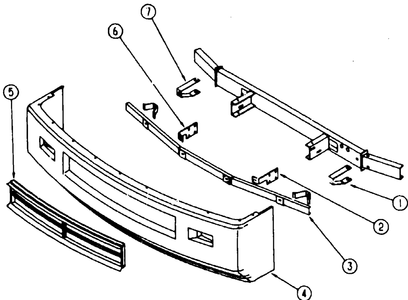
FRONT BUMPER
