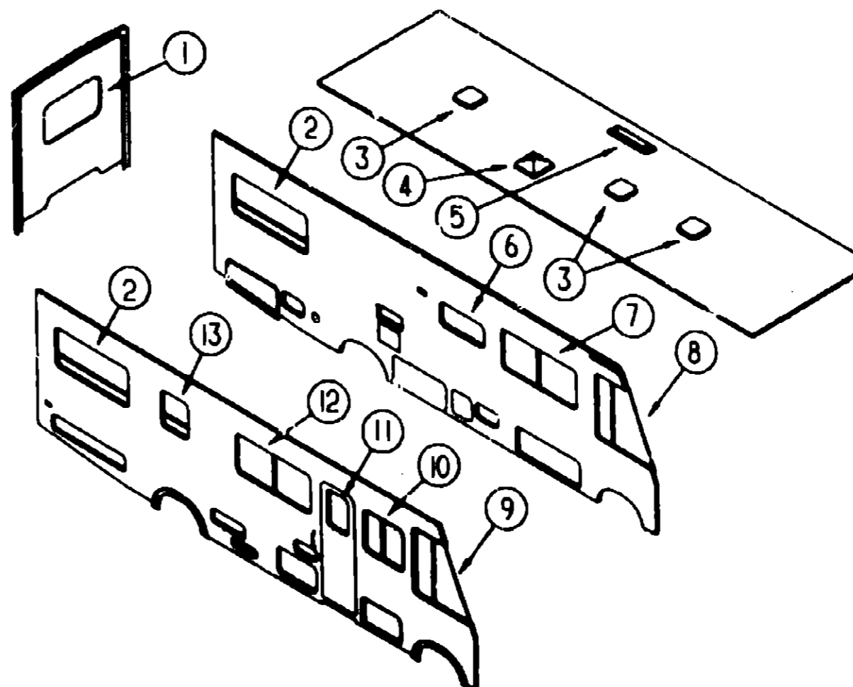
WINDOWS & VENTS
