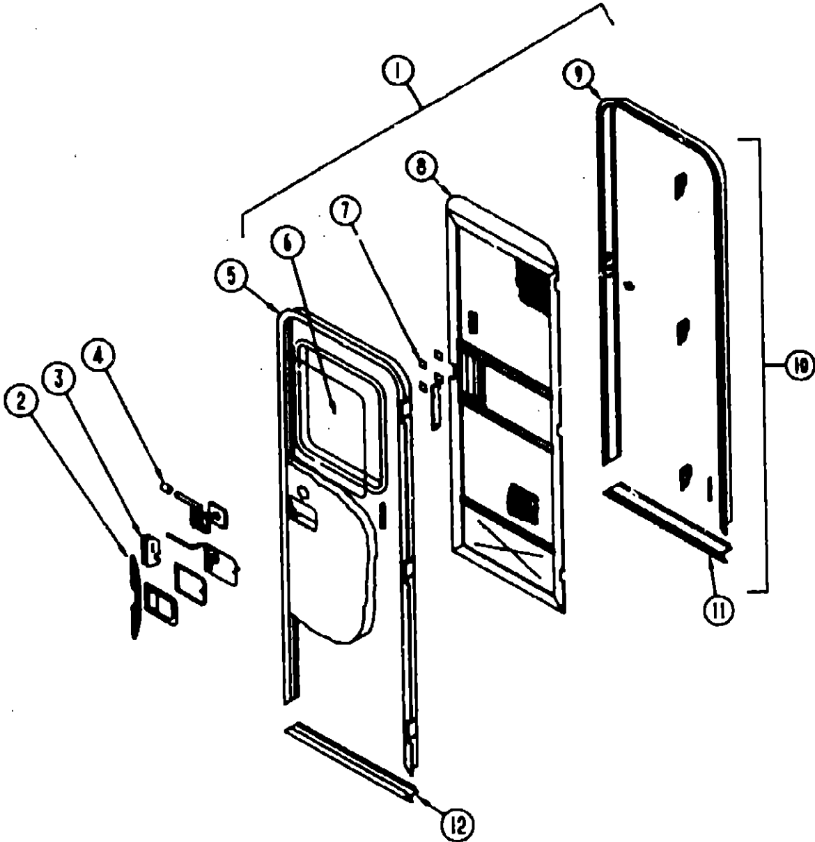
ENTRANCE DOOR
