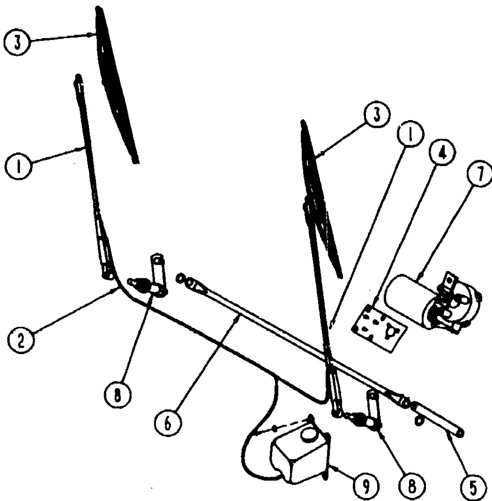
WIPER COMPONENTS
