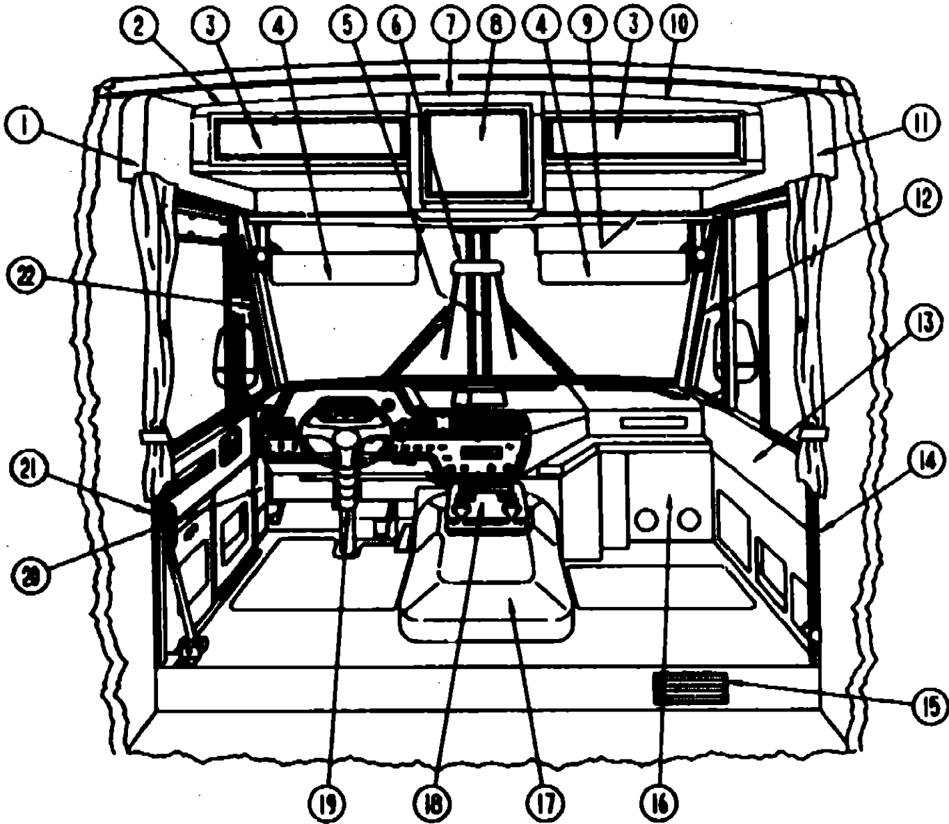
DRIVERS COMPARTMENT
