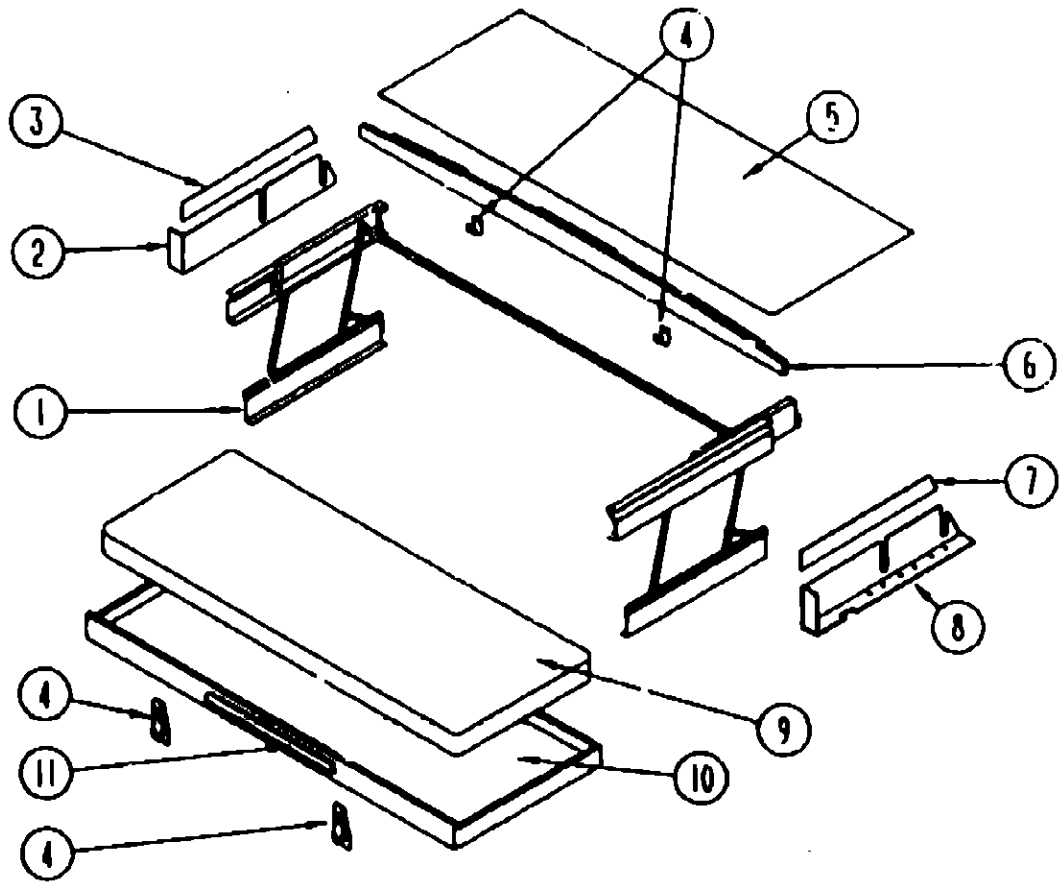
FRONT BUNK-SINGLE
