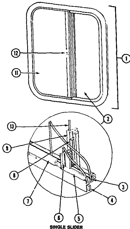
SINGLE SLIDER
