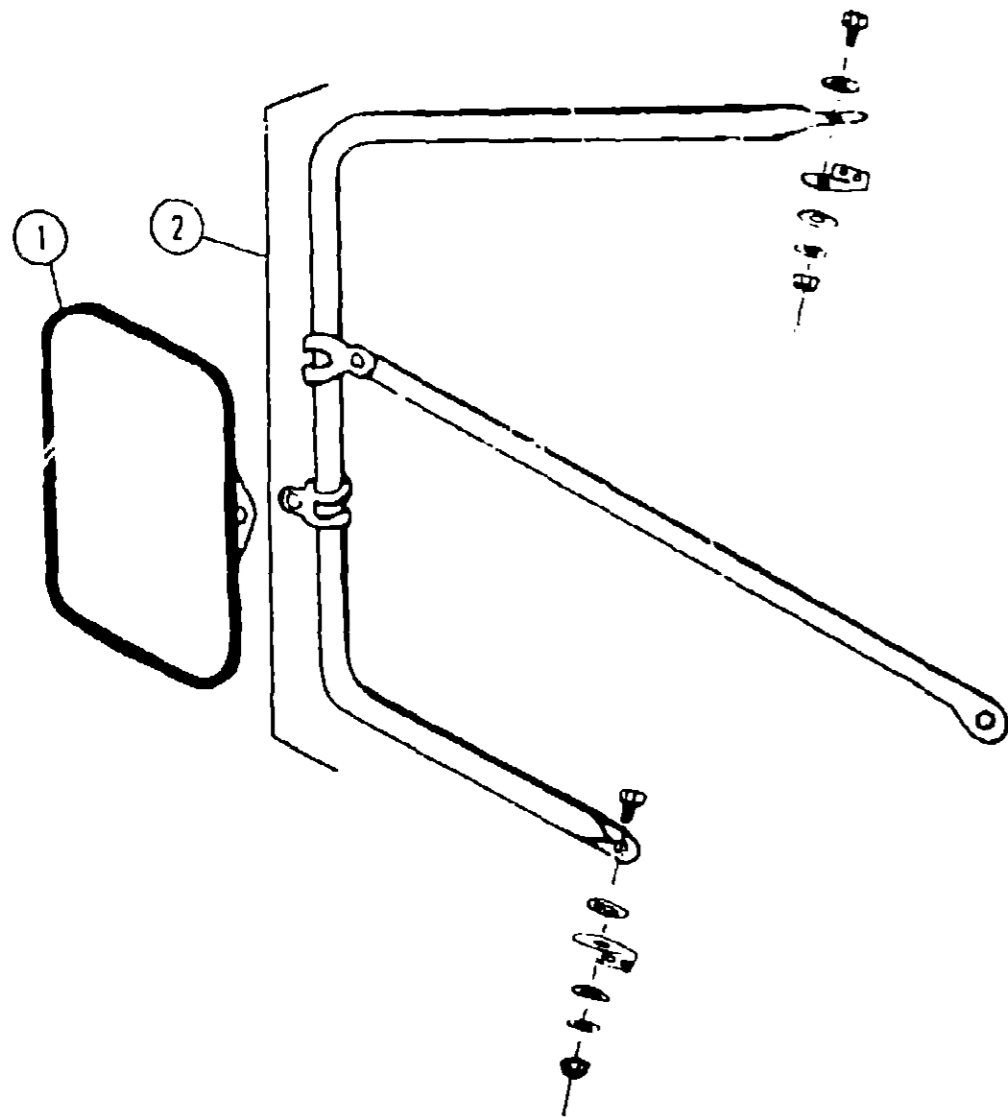
EXTERIOR MIRRORS
