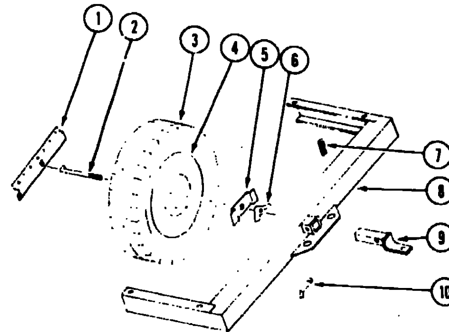
SPARE TIRE CARRIER & TRAILER HITCH
