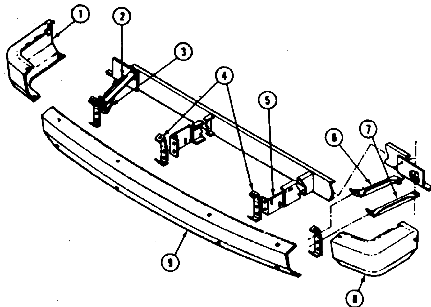
FRONT BUMPER
