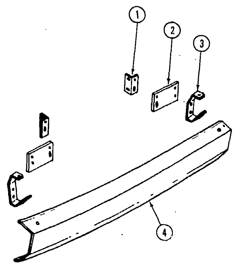
REAR BUMPER
