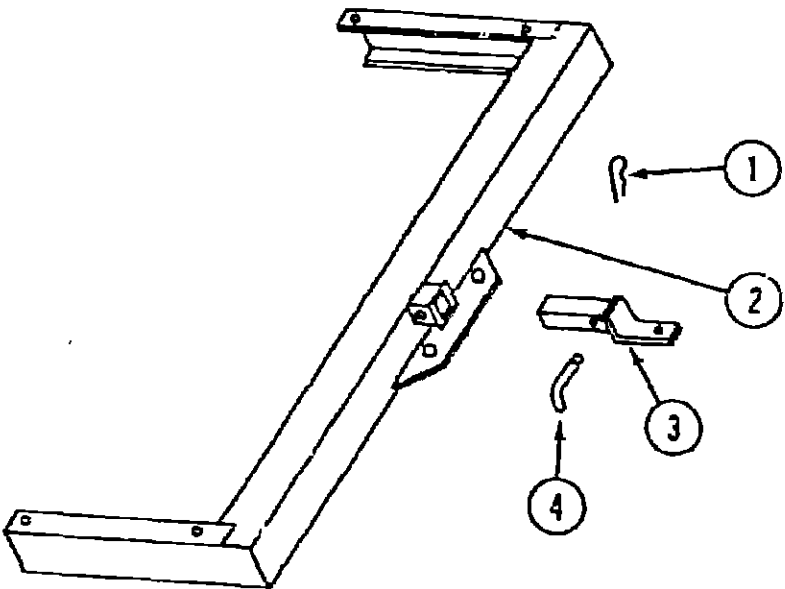
TRAILER HITCH
