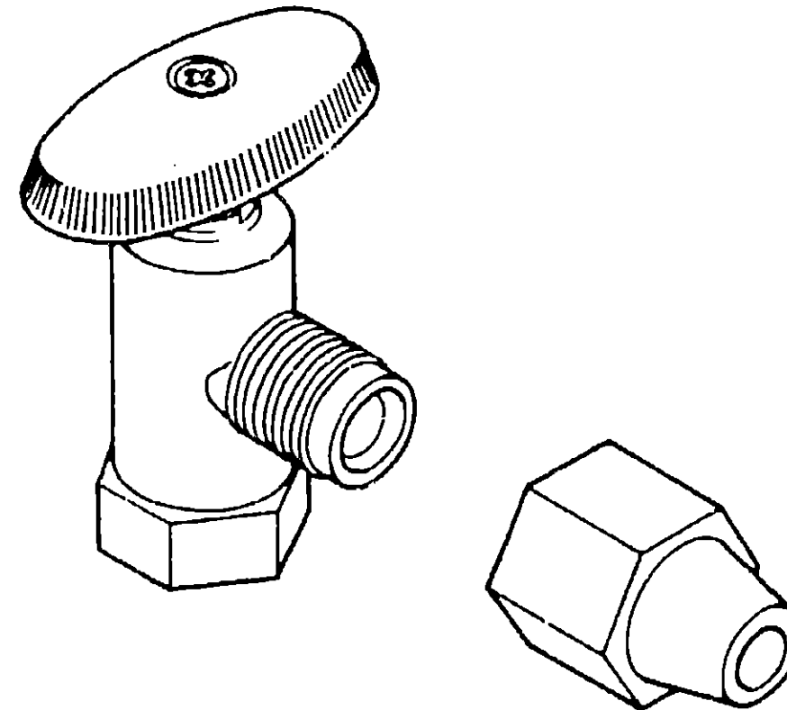
Key Part Number U/M Description 03PJ09-01-000 EA Stool Valve - Plastic - 3/8" C x 1/2" FPT
