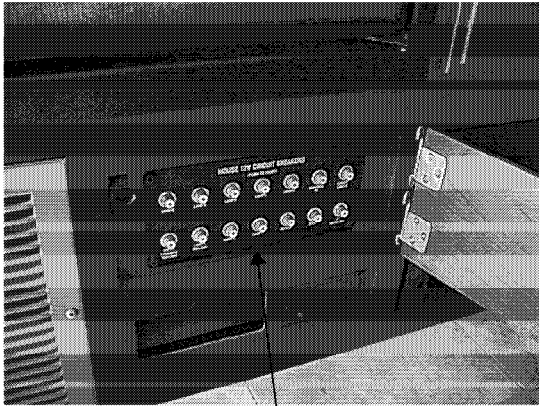
House 12V Breakers
