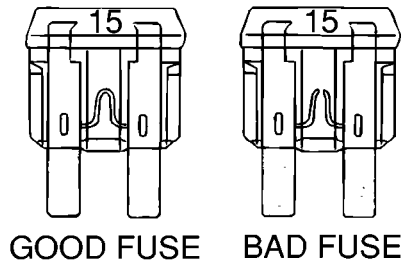
PLUG-IN FUSES
