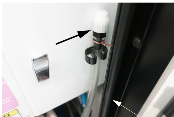
Antifreeze Siphon Tube attached to the tank fill inlet -Typical View
