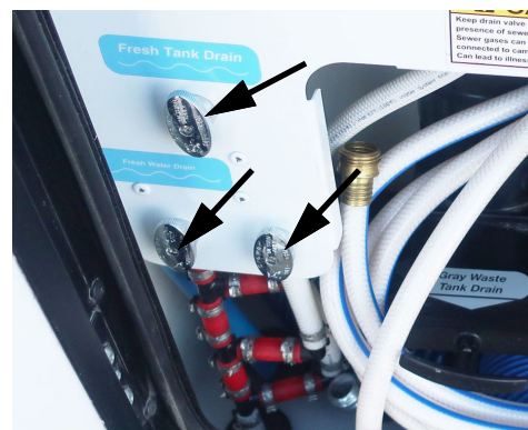
Open 3 of the General Waterline drain valves located at the Water Service Center (Shown in the open position). -Typical View
