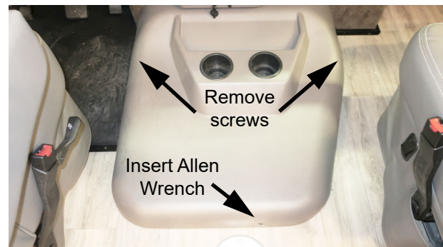
Motor Cover Allen Wrench (Located in the InfoCase)
