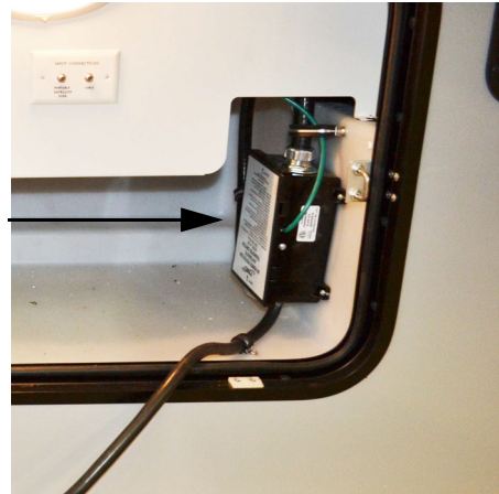
Automatic Power Transfer Box (Located inside water service center compartment) -Typical installation shown
