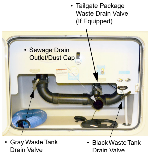
Holding Tank Drain Valves (Located in water service center) *Model 29V
