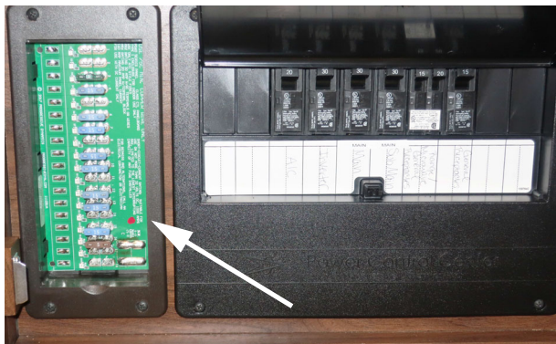
House 12-Volt Fuses (Located on Power Converter) -Typical View
