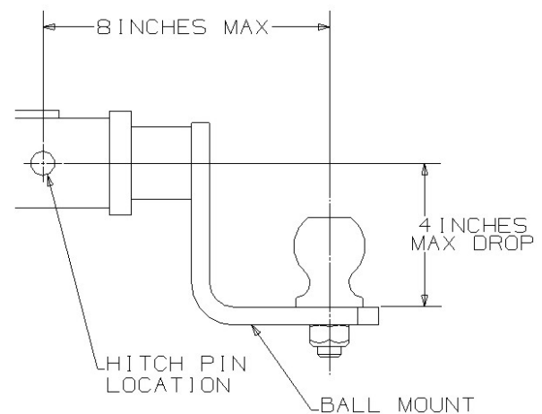
Hitch Assembly
