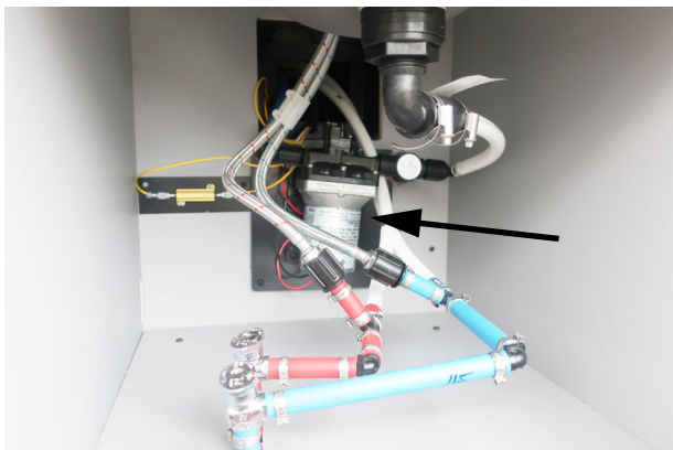
Exterior Sink Pump (Located in the passenger side compartment behind rear axle) -Typical View
