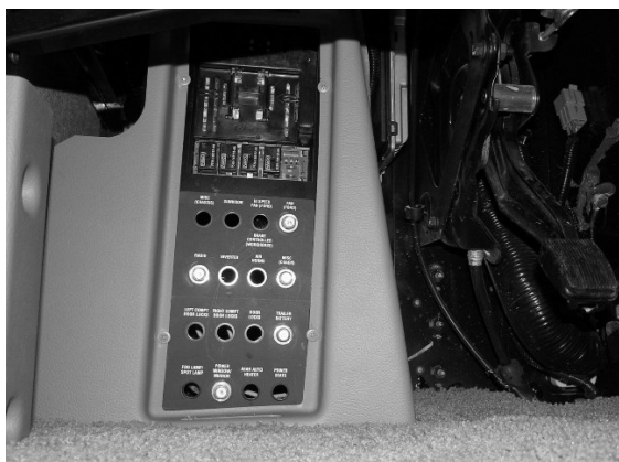
Automotive 12-Volt Circuit Breakers and Fuses (Located beneath left end of dash) -Typical View
