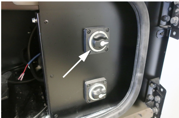
250 Amp Circuit Breaker (Located in the passenger side compartment) (Option 33W shown) -Typical view
