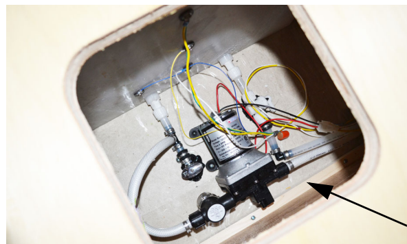
Water Pump (Located beneath bed - lift mattress to expose access hole) *Models 22R, 25B, 31H, and 31K -Typical View
