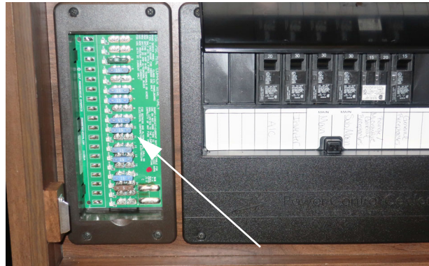
House 12-Volt Fuses (Located near Power Converter) -Typical View
