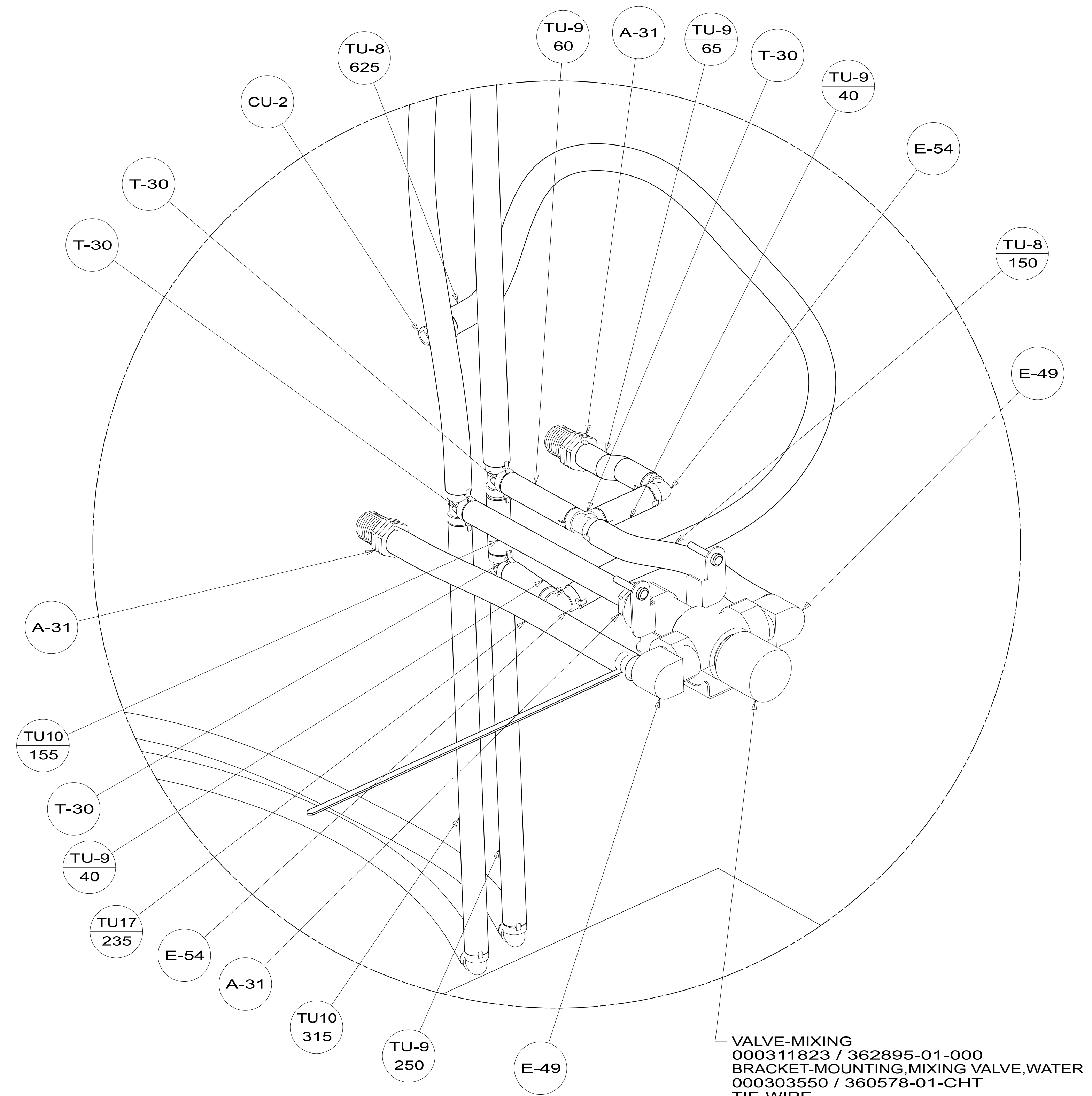
DETAIL BB
