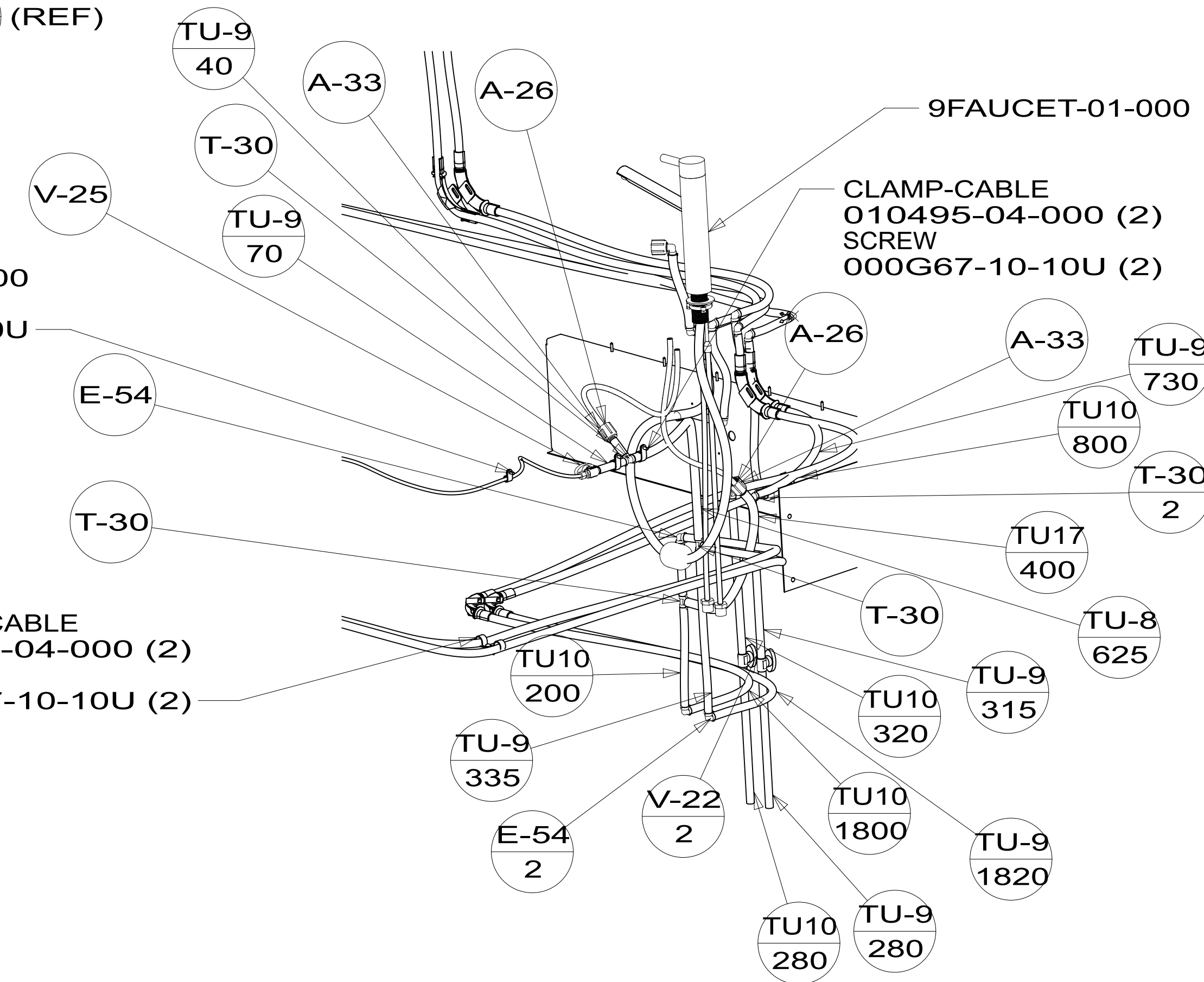
DETAIL EC
