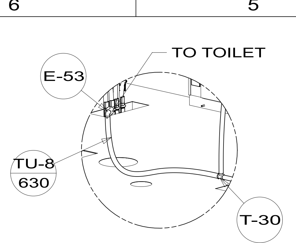
DETAIL BF
