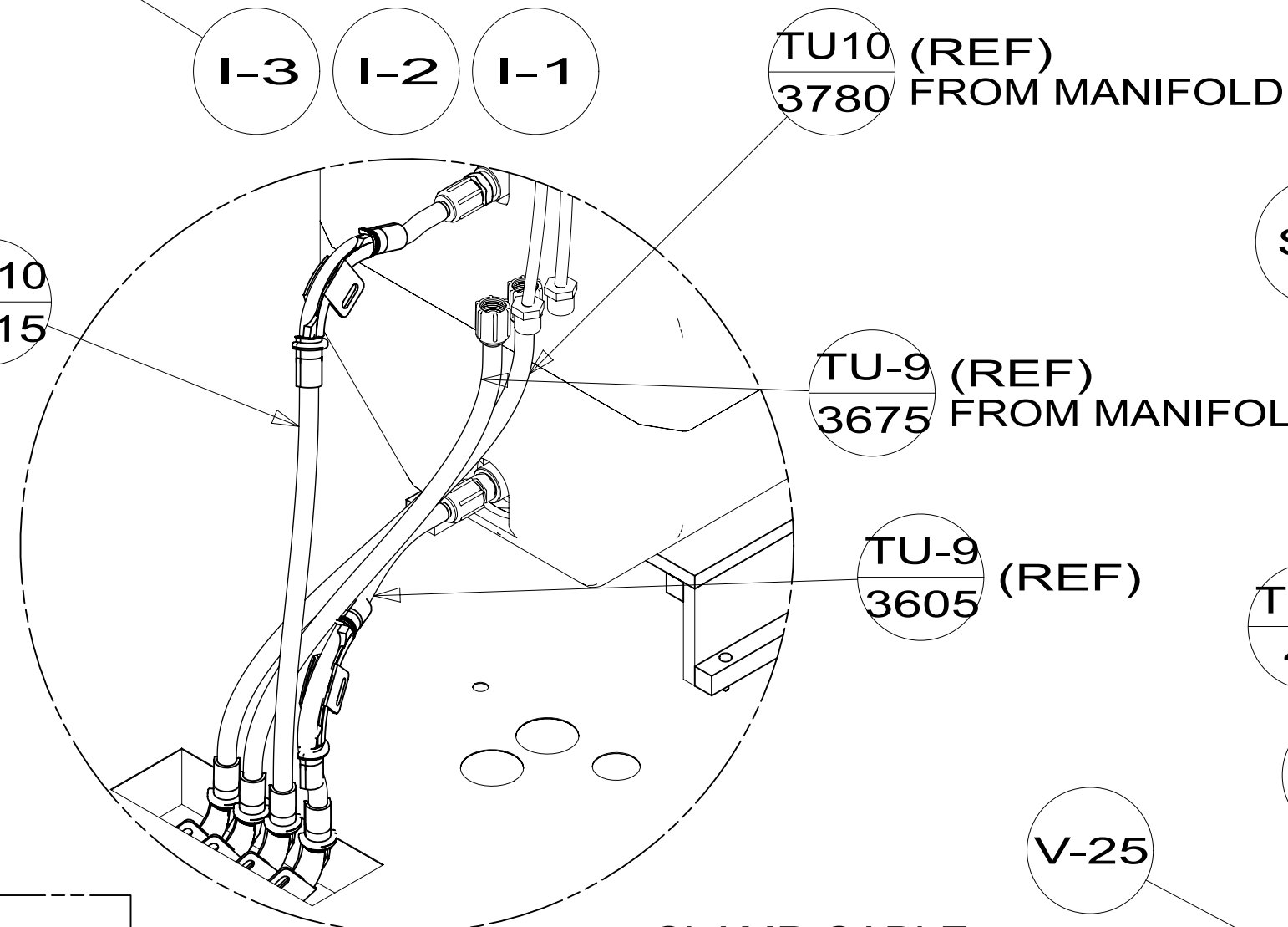
DETAIL EF
