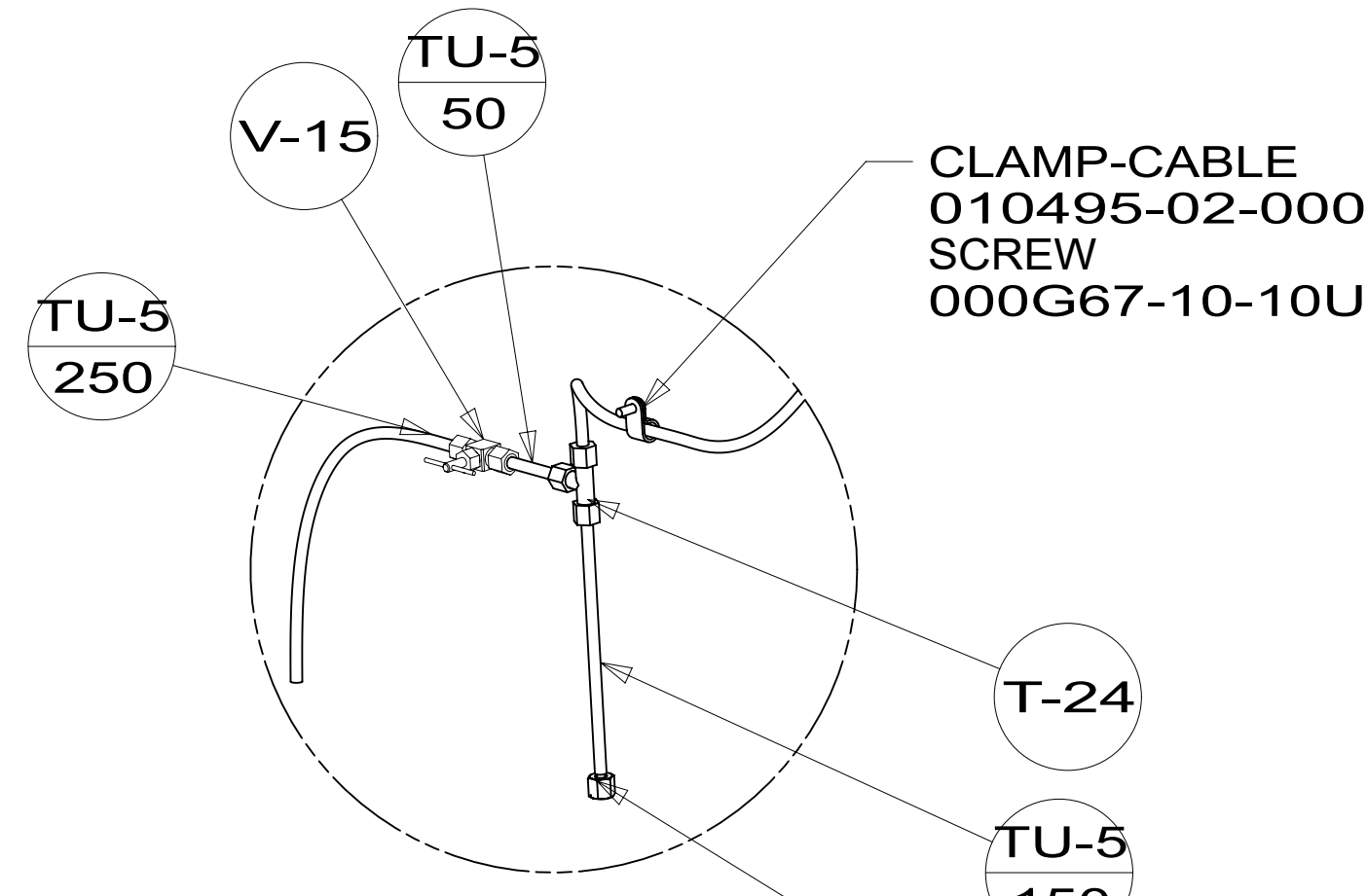
DETAIL EE
