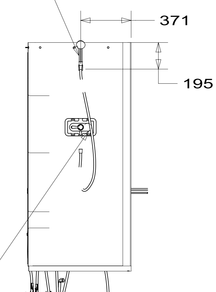
SECTION BD-BD
