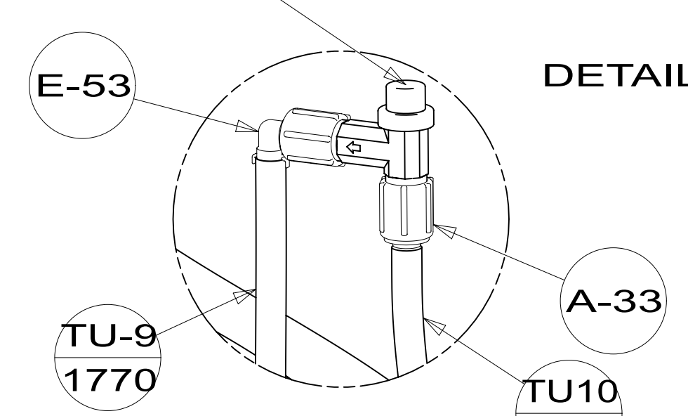
DETAIL BE
