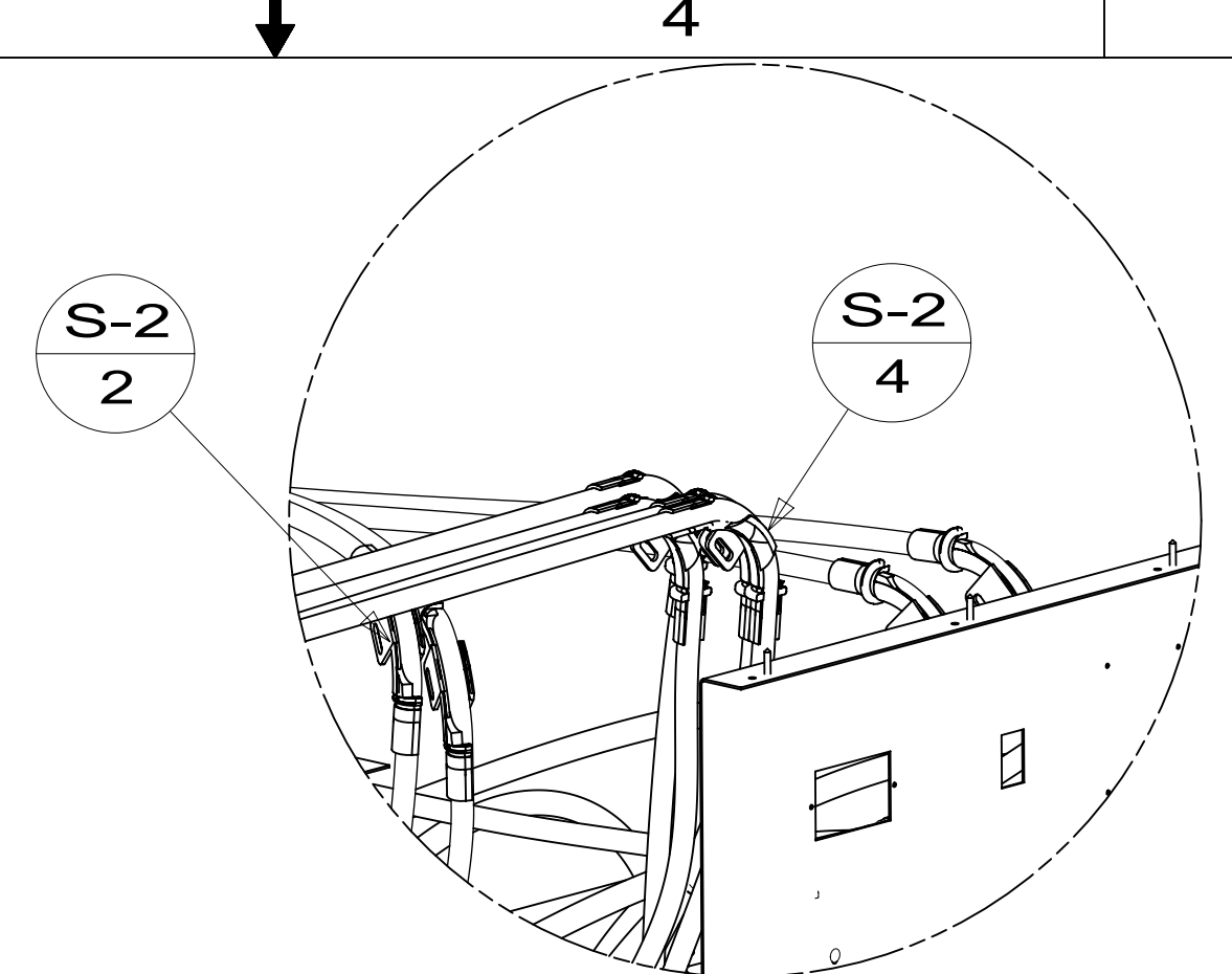
DETAIL BK
