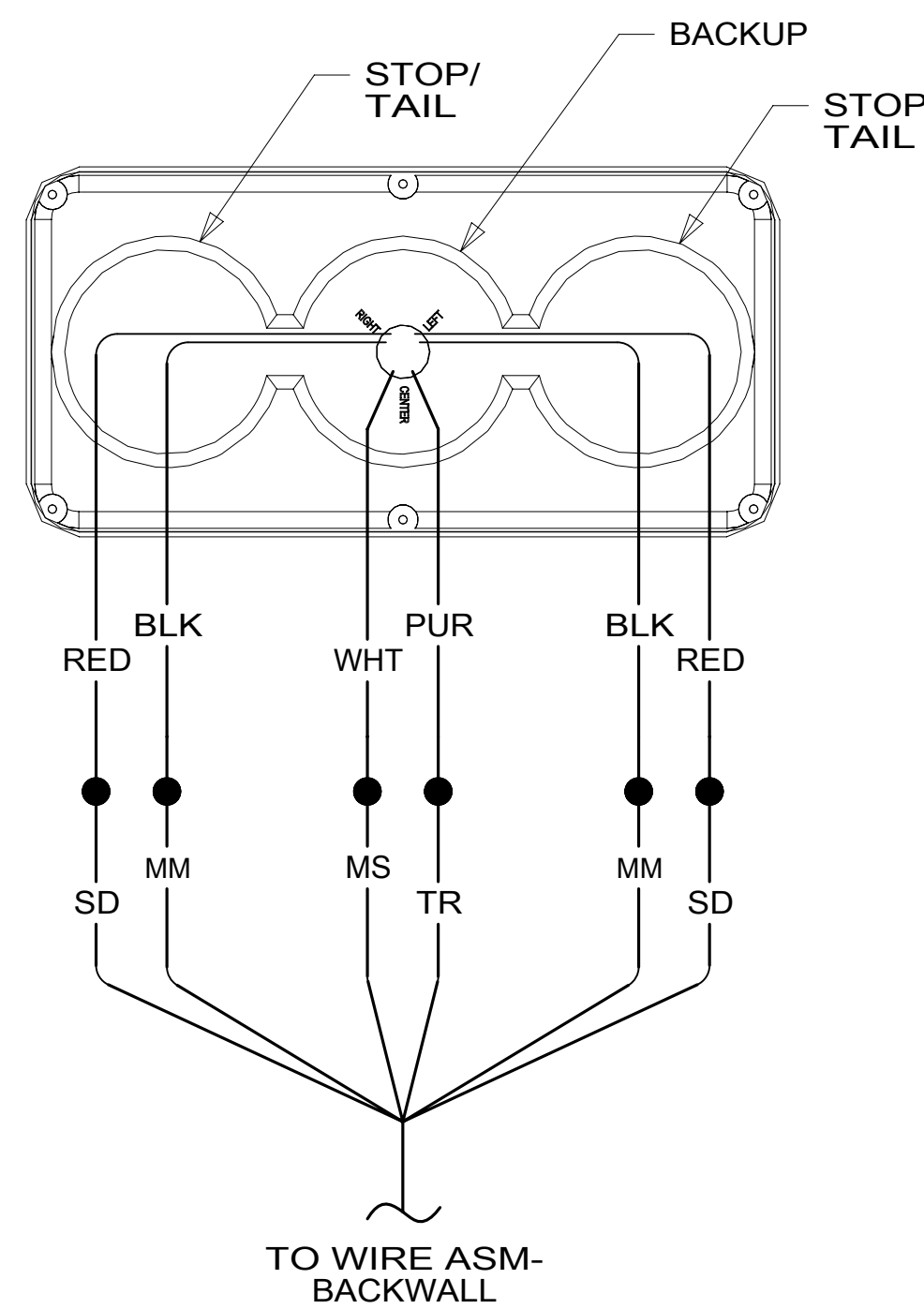
DETAIL BC
