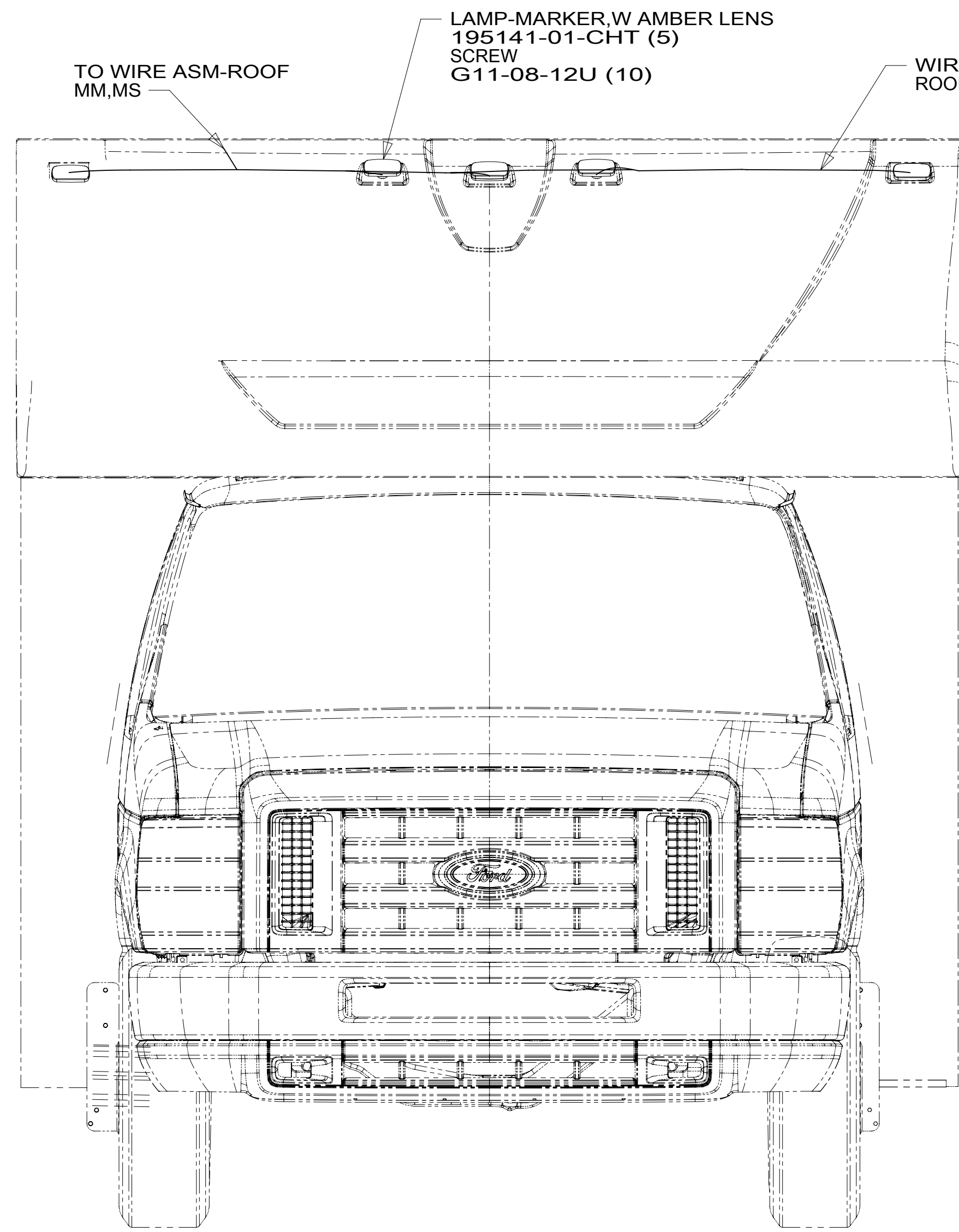
VIEW BA
