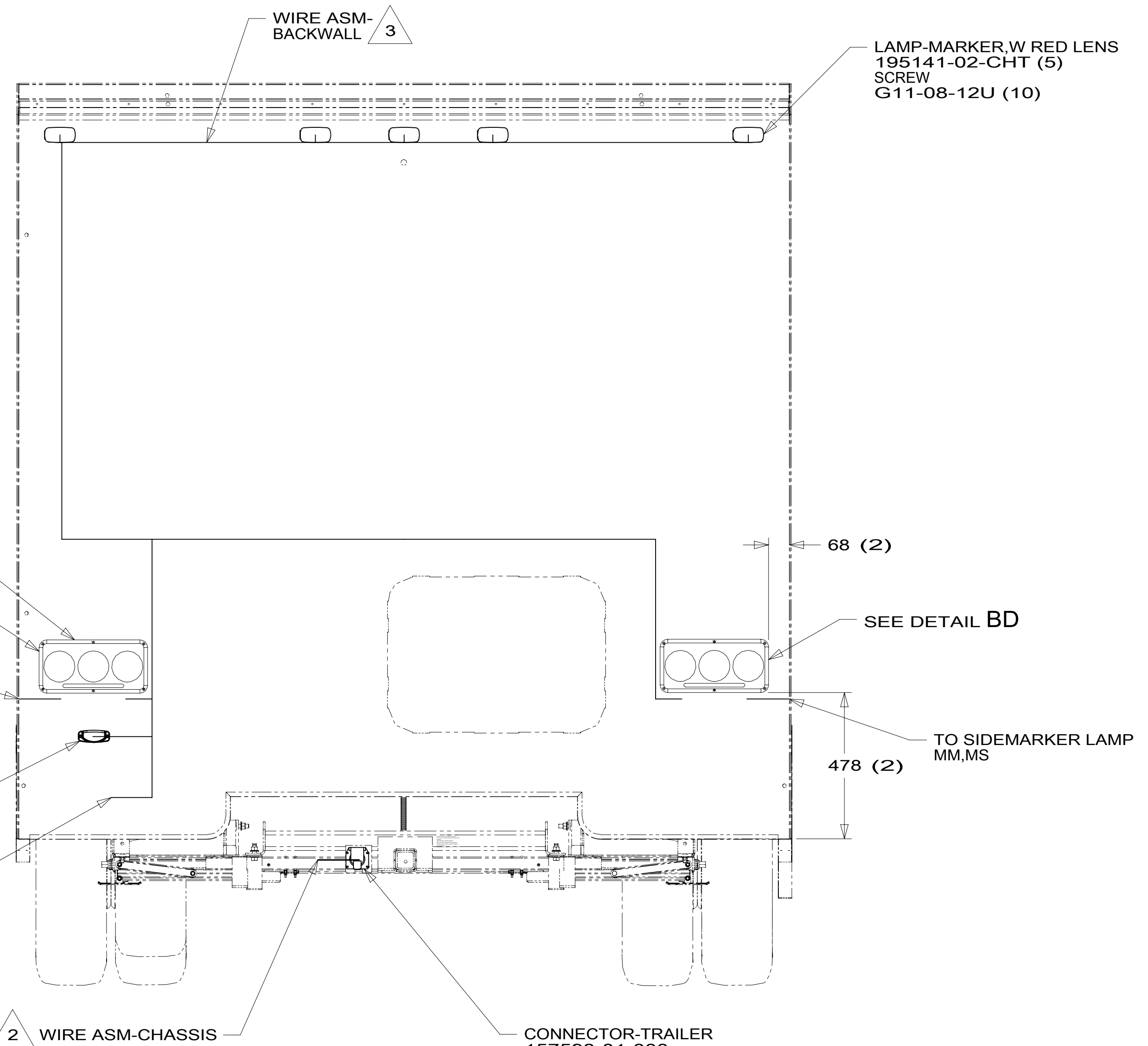
VIEW BB
