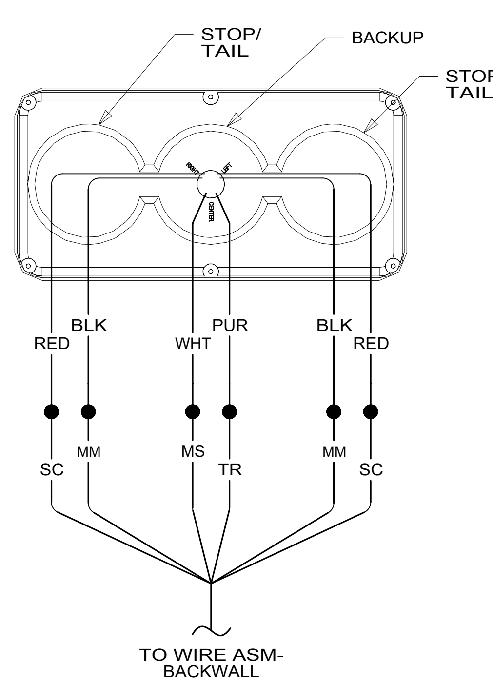
DETAIL BD
