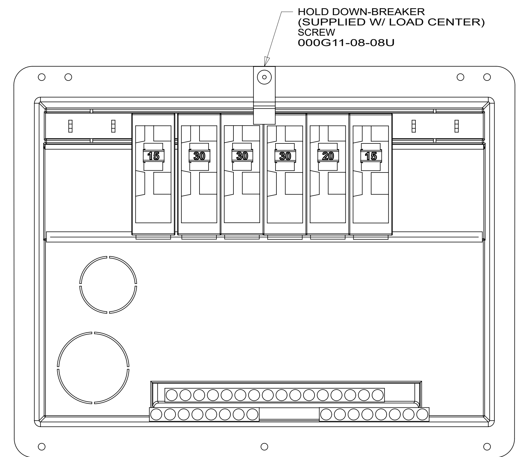
FRONT VIEW (FRONT COVER REMOVED)
