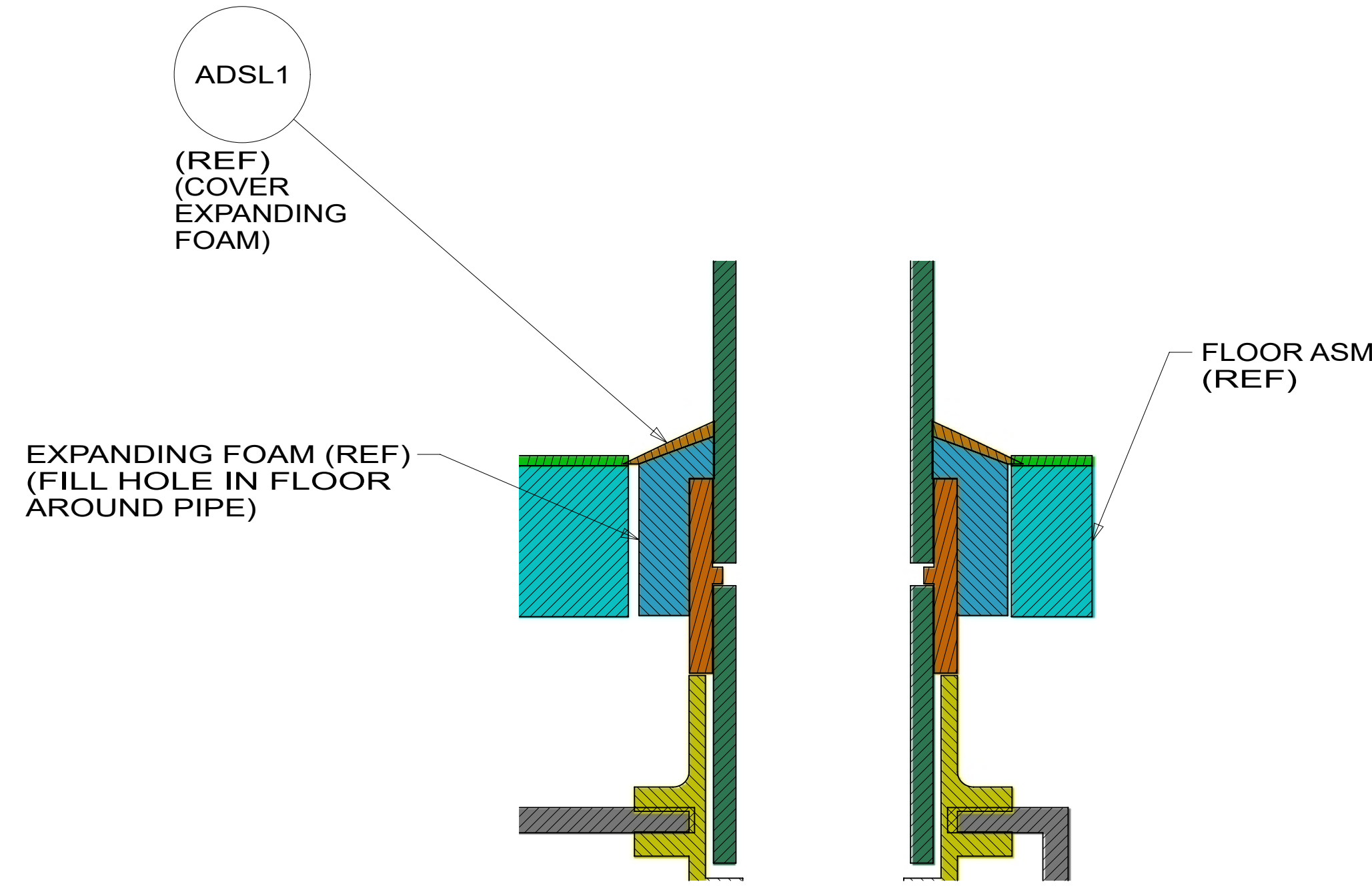
SECTION CG-CG
