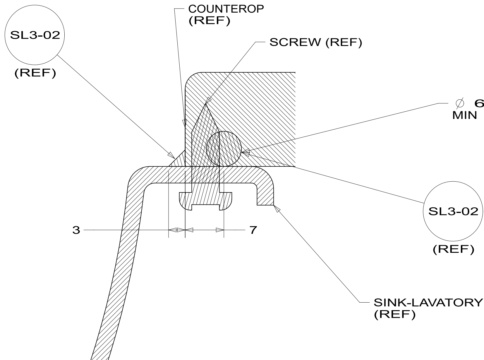
SECTION CF-CF
