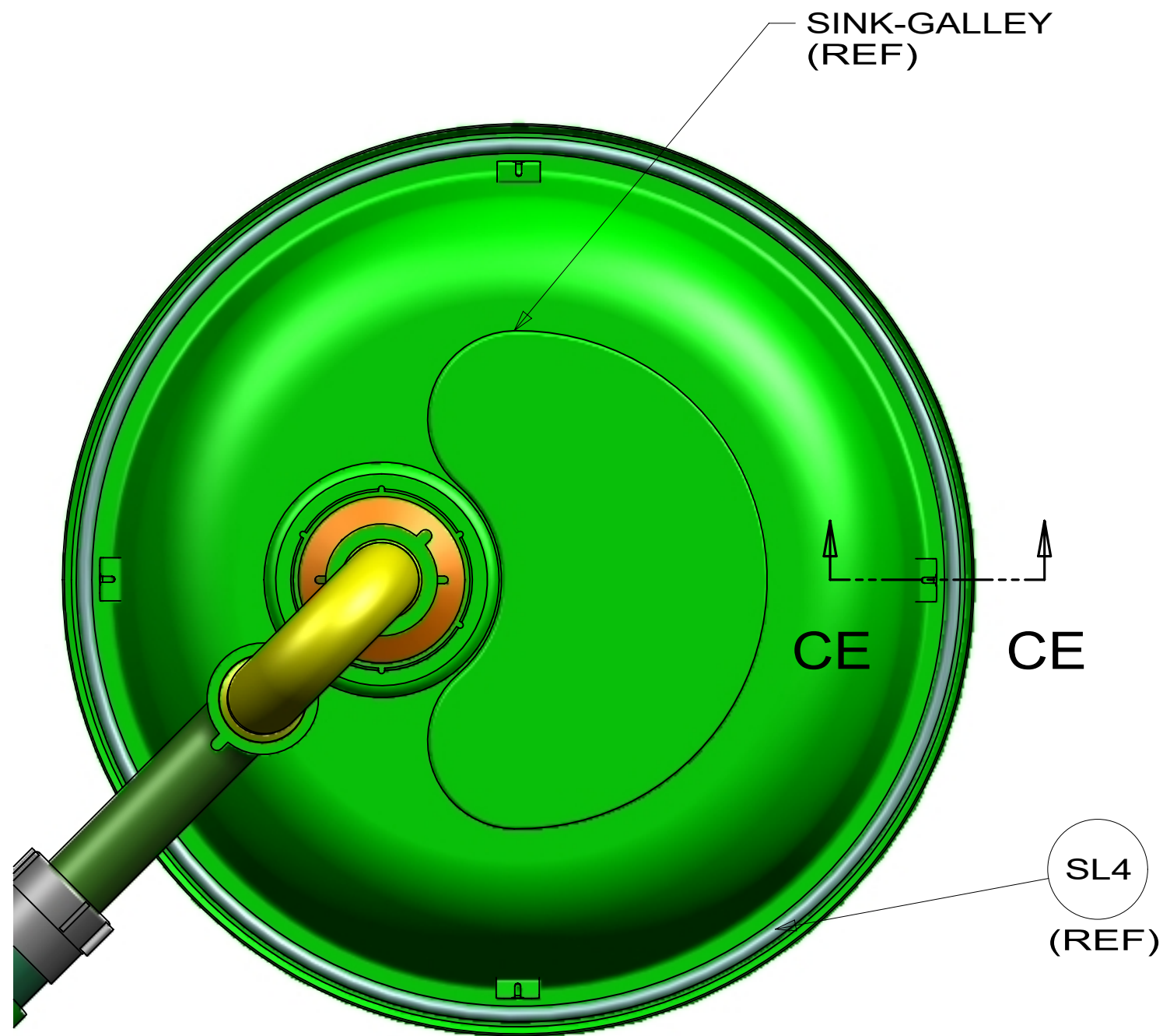
VIEW CC
