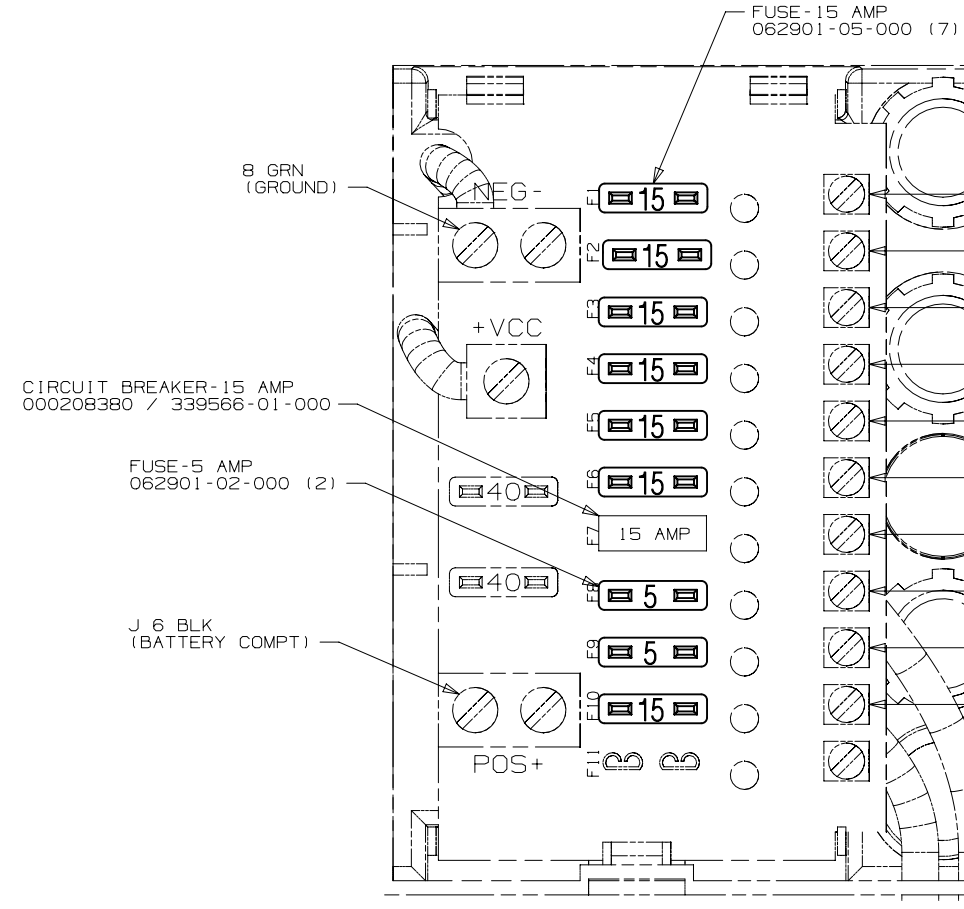
DETAIL CH
