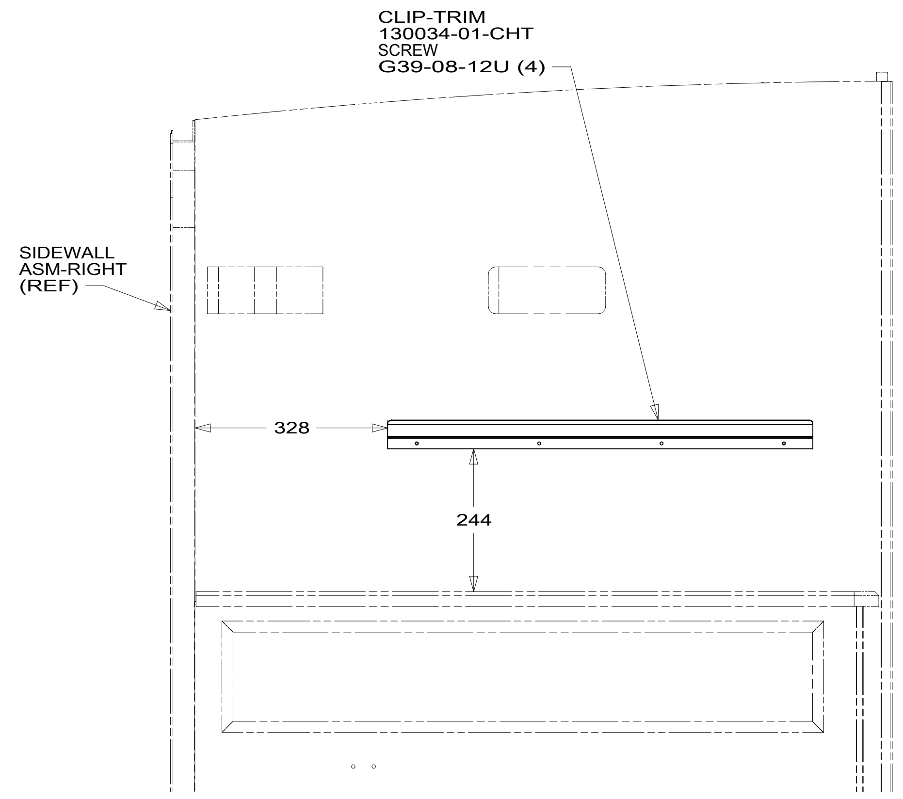
VIEW BA (TV NOT SHOWN)
