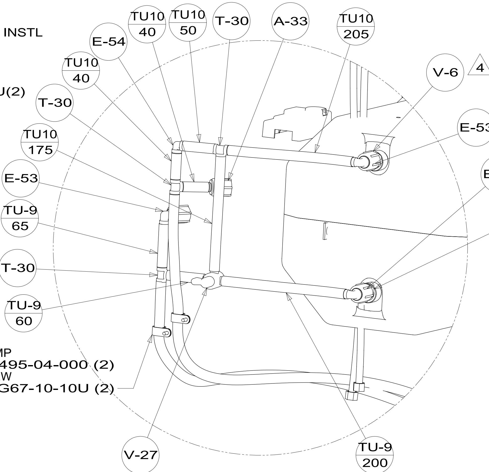
DETAIL BB (SHOWN W/OUT CABINETS)
