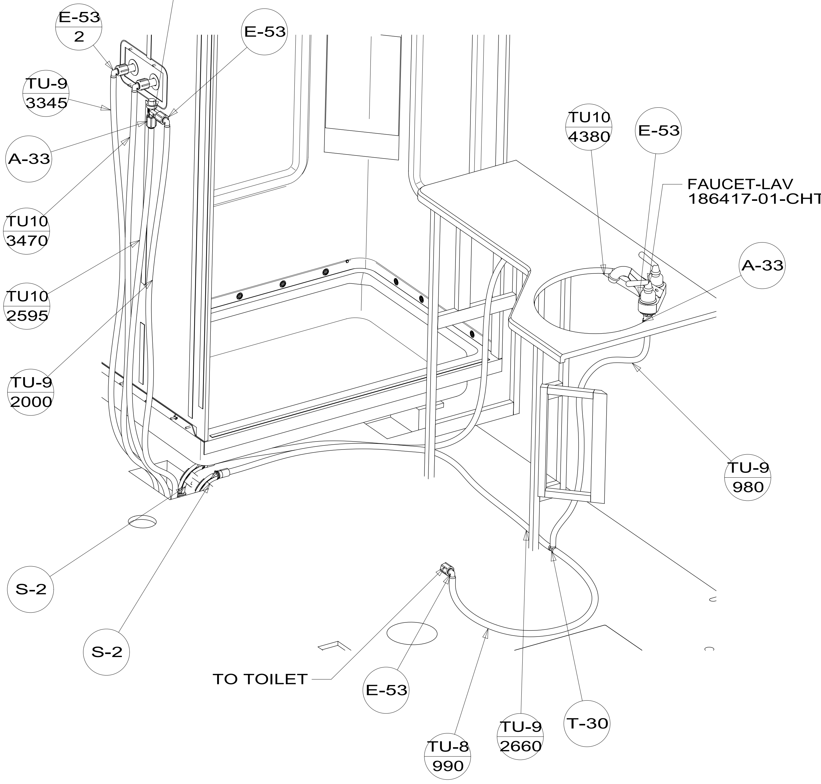
VIEW BC
