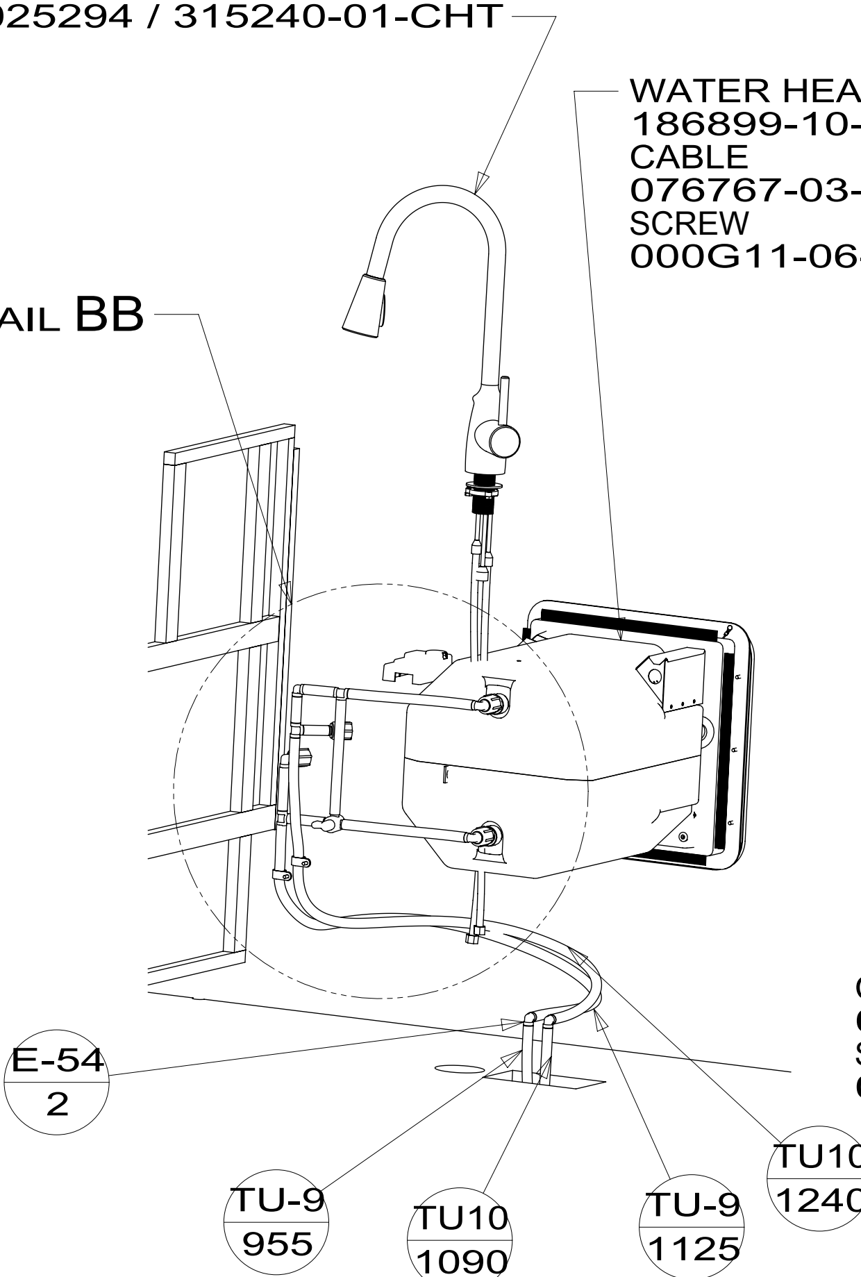
VIEW BA
