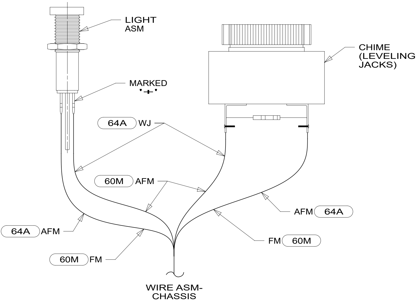
DETAIL HC
