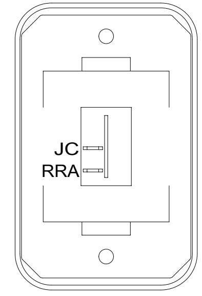
DETAIL DJ
