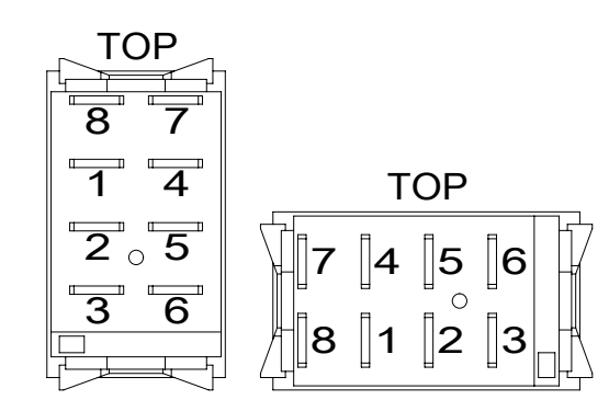
DETAIL DP
