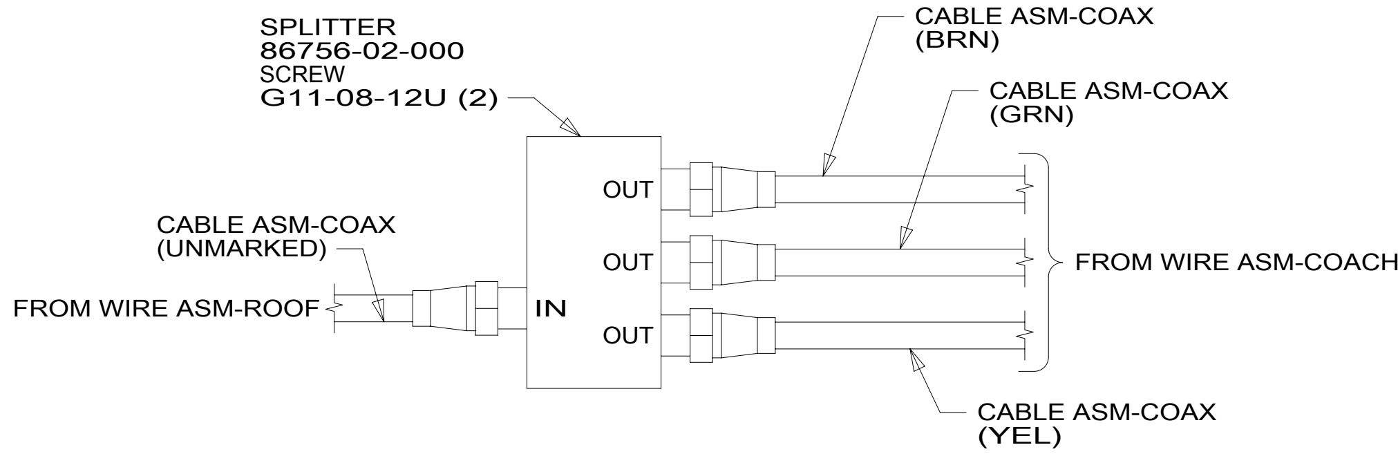
DETAIL DG
