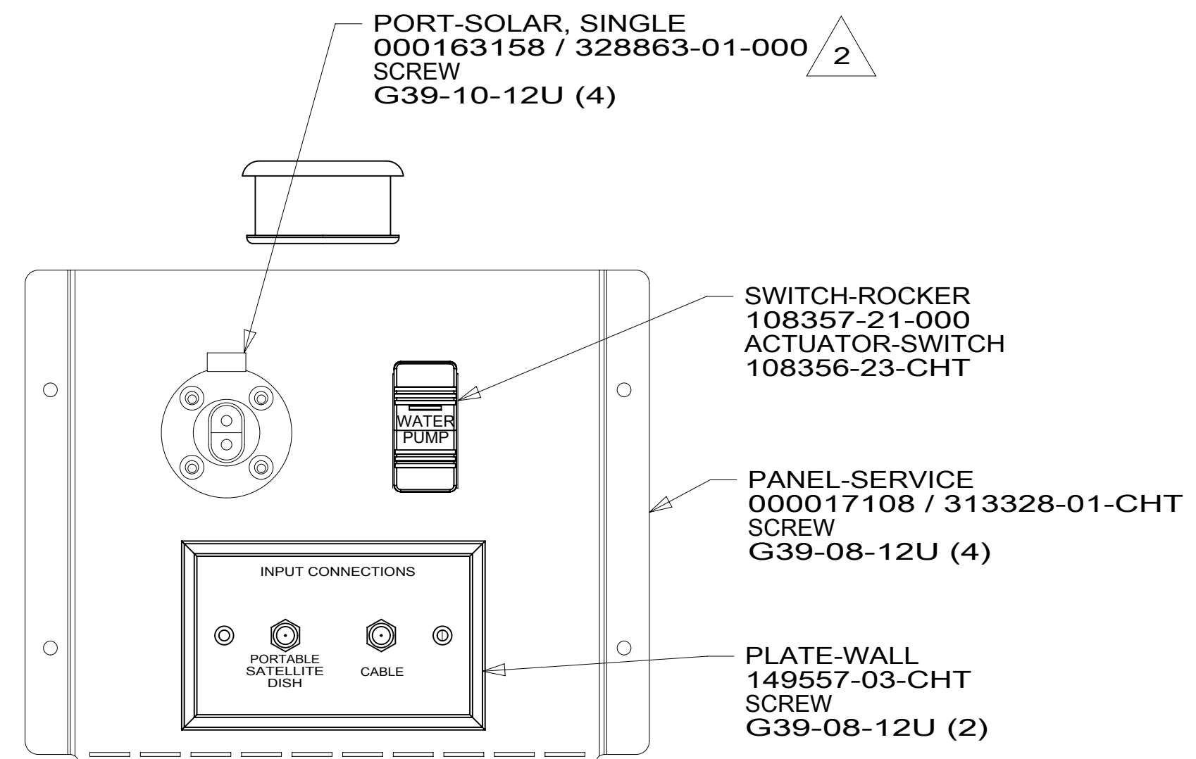
VIEW AA
