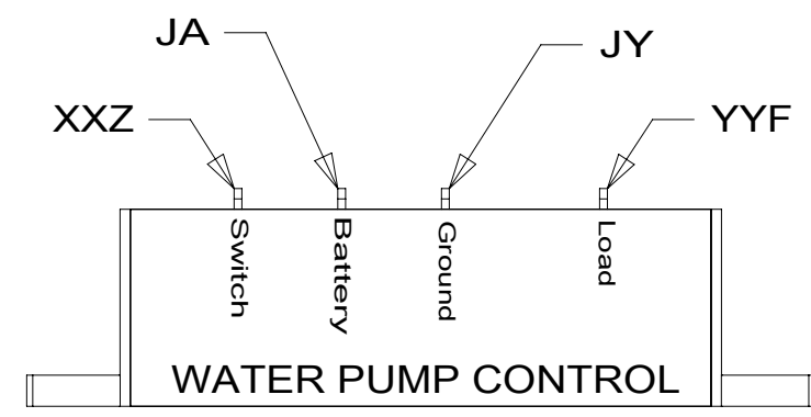
DETAIL DJ
