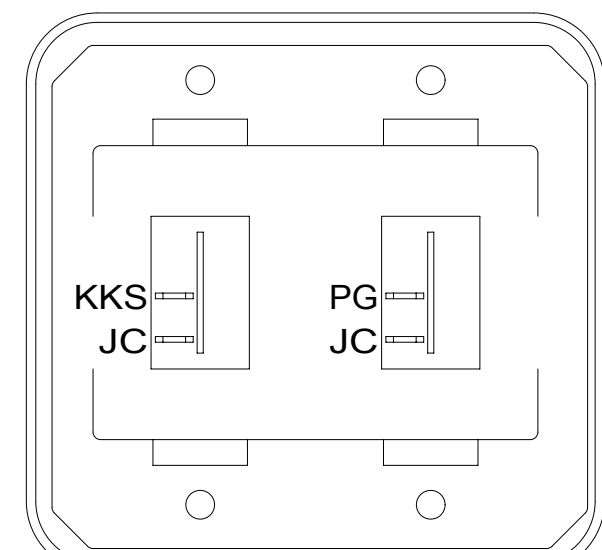
DETAIL DL
